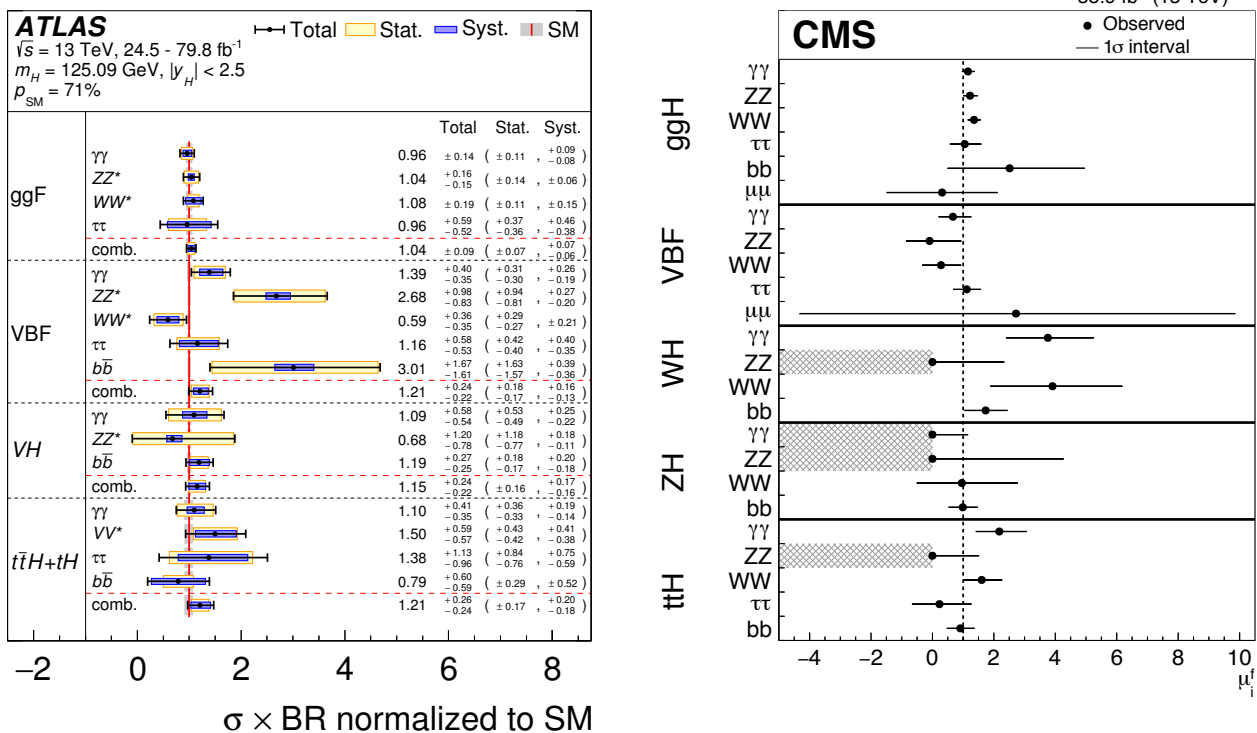
Figure 11.8: Combined measurements of the products \sigma \cdot \text{BR} , normalised to the SM predictions, for the five main production and five main decay modes. The hatched combinations require more data for a meaningful confidence interval to be provided.
