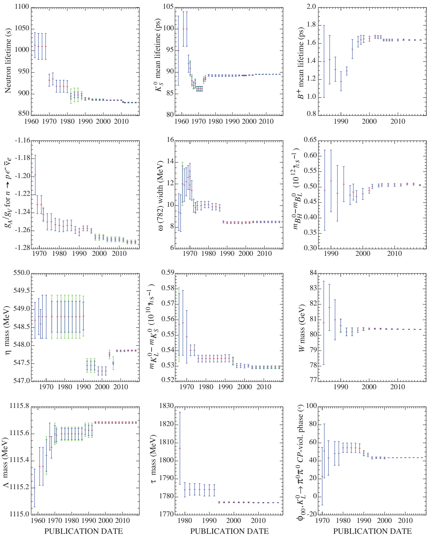
Figure 1: A historical perspective of values of a few particle properties tabulated in this Review as a function of date of publication of the Review . A full error bar indicates the quoted error; a thick-lined portion indicates the same but without the “scale factor.”
