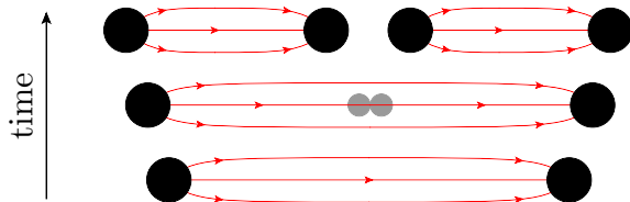
Figure 42.2: Illustration of string breaking by quark pair-creation in the string field.
