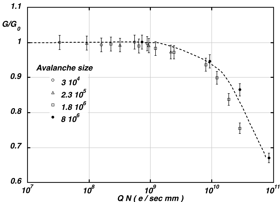
Figure 35.8: Charge rate dependence of normalized gas gain G/G_0 (relative to zero counting rate) in proportional thin-wire detectors [111]. Q is the total charge in single avalanche; N is the particle rate per wire length.
