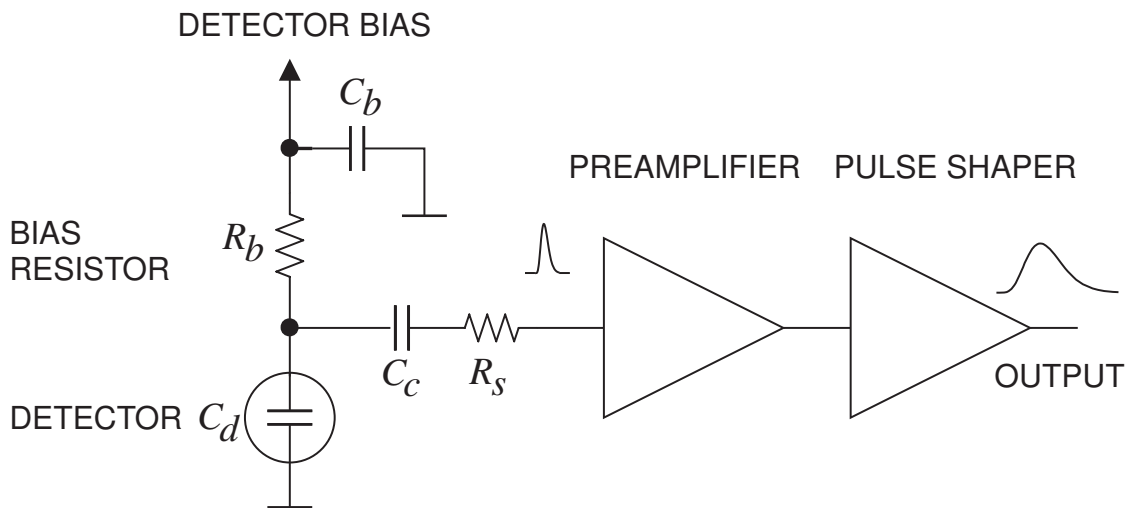
Figure 35.18: Typical detector front-end circuit.
