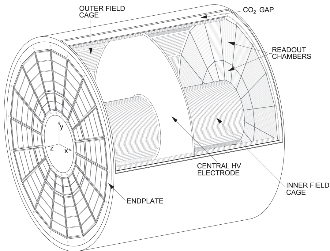
Figure 35.13: Schematic view of the ALICE TPC [133]. The drift volume with 5 m diameter is divided into two halves, each providing 2.5 m drift length.
