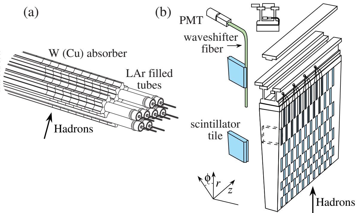
Figure 35.22: (a) ATLAS forward hadronic calorimeter structure (FCal2, 3) [212]. Tubes containing LAr are embedded in a mainly tungsten matrix. (b) ATLAS central calorimeter wedge; iron with plastic scintillator tile with wavelength-shifting fiber readout [213].
