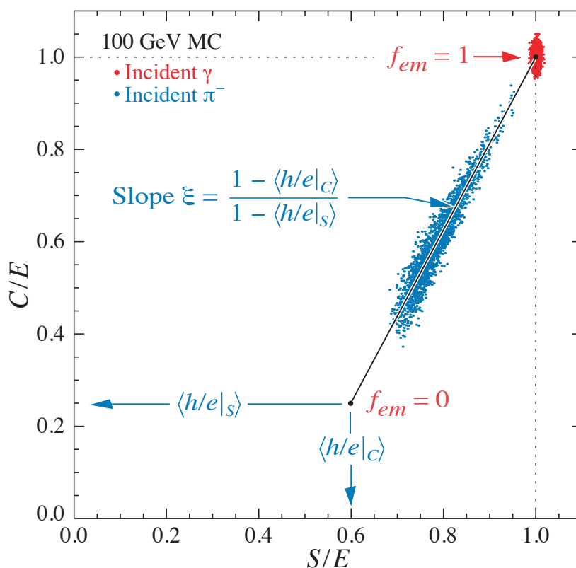
Figure 35.23: Scatter plot of Monte Carlo C/E (Cherenkov) vs S/E (scintillator) signals for individual events in a dual readout calorimeter. Hadronic events are shown in blue, and scatter about the indicated event locus. Electromagnetic events cluster about (C/E, S/E) = (1,1) . In this case worse resolution (fewer p.e.'s) was assumed for the Cherenkov events, leading to the “elliptical” distribution.
