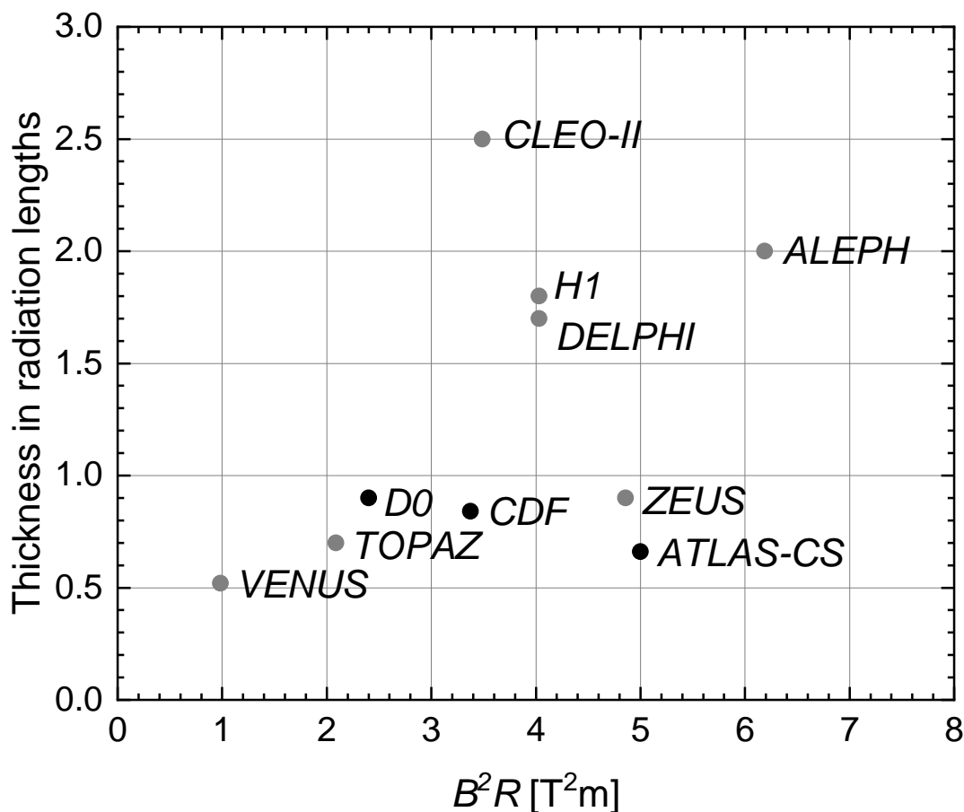
Figure 35.26: Magnet wall thickness in radiation length as a function of B^2R for various detector solenoids. Gray entries are for magnets no longer in use, and entries underlined are not listed in Table 35.11. Open circles are for magnets not designed to be “thin.” The SSC-SDC prototype provided important R&D for LHC magnets.
