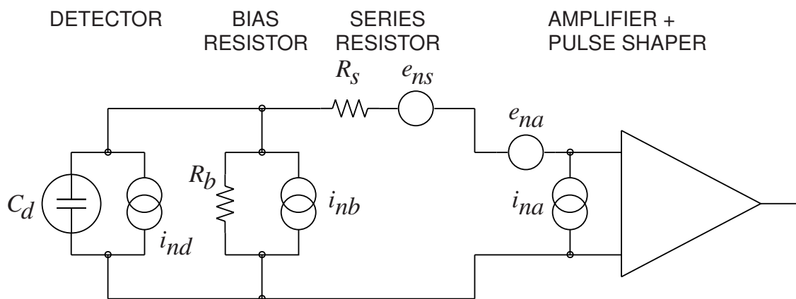
Figure 35.19: Equivalent circuit for noise analysis.
