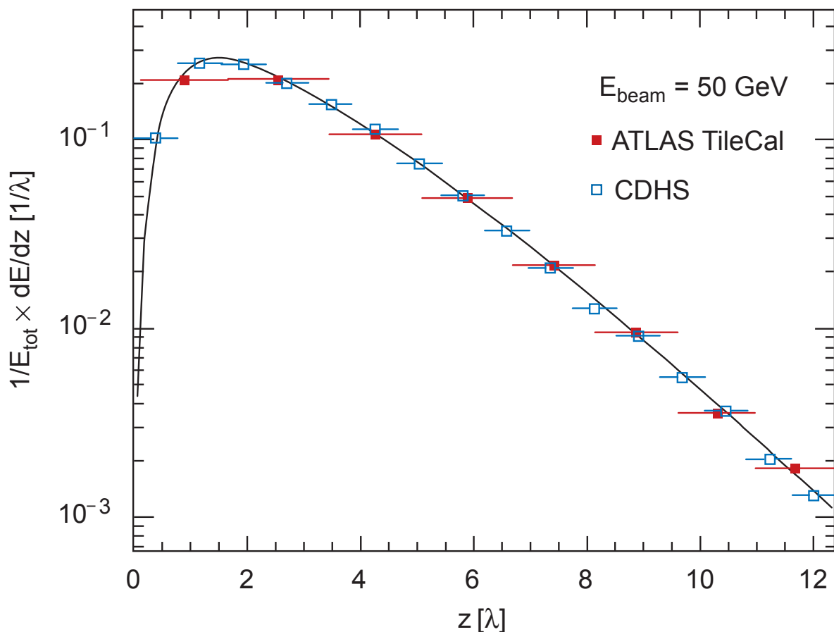
Figure 35.24: Mean profiles of \pi^+ (mostly) induced cascades in the CDHS neutrino detector [255] and in the ATLAS tile calorimeter [224]. Measurements are front of the calorimeter, and so are convoluted with the first interaction distance.
