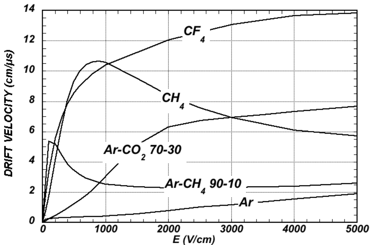
Figure 35.4: Computed electron drift velocity as a function of electric field in several gases at NTP and B = 0 [87].
