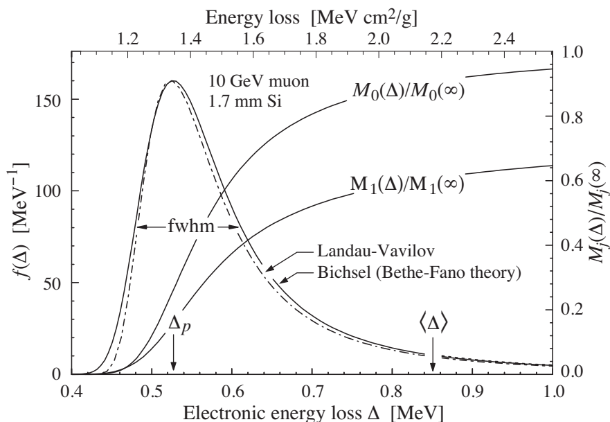
Figure 34.7: Electronic energy deposit distribution for a 10 GeV muon traversing 1.7 mm of silicon, the stopping power equivalent of about 0.3 cm of PVT-based scintillator [1, 11, 32]. The Landau-Vavilov function (dot-dashed) uses a Rutherford cross section without atomic binding corrections but with a kinetic energy transfer limit of W_{\max} . The solid curve was calculated using Bethe-Fano theory. M_0(\Delta) and M_1(\Delta) are the cumulative 0th moment (mean number of collisions) and 1st moment (mean energy loss) in crossing the silicon. (See Sec. 34.2.1). The fwhm of the Landau-Vavilov function is about 4\xi for detectors of moderate thickness. \Delta_p is the most probable energy loss, and \langle\Delta\rangle divided by the thickness is the Bethe \langle dE/dx\rangle .
