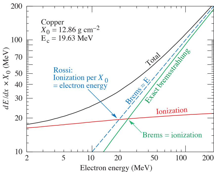
Figure 34.13: Two definitions of the critical energy E_c .
