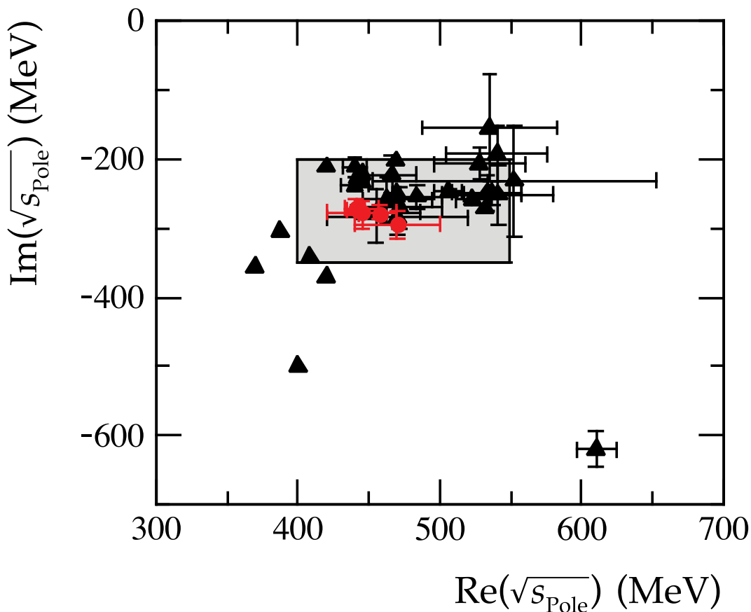
Figure 62.2: Location of the f_0(500) (or \sigma ) poles in the complex energy plane. Circles denote the recent analyses based on Roy(-like) dispersion relations, while all other analyses are denoted by triangles. The corresponding references are given in the listing.
