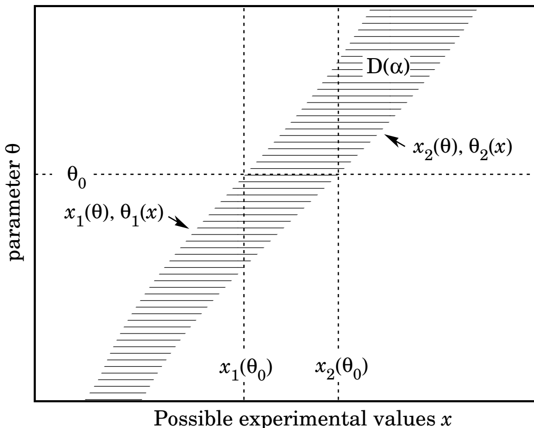
Figure 40.3: Construction of the confidence belt (see text).
