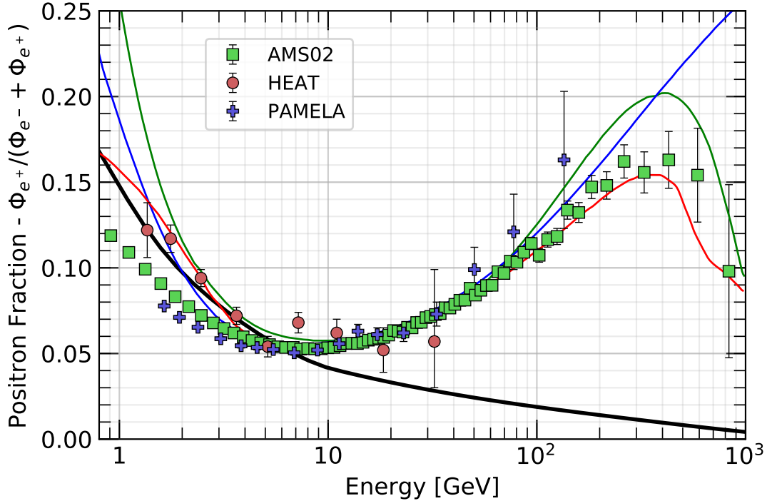
Figure 30.4: The positron fraction (ratio of the flux of e^+ to the total flux of e^+ and e^- ) [33,41,42,46]. The heavy black line is a model of pure secondary production [45] and the three thin lines show three representative attempts to model the positron excess with different phenomena: green: dark matter decay [49]; blue: propagation physics [48]; red: production in pulsars [63]. The ratio below 10 GeV is dependent on the intensity and polarity of the solar magnetic field.
