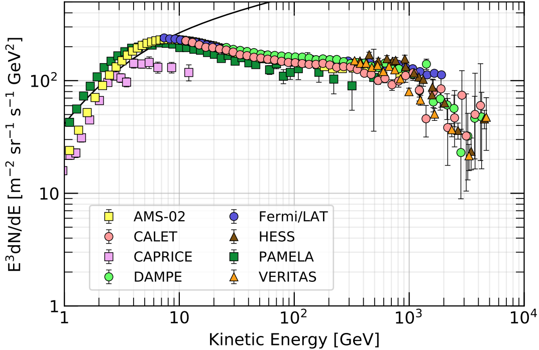
Figure 30.3: Differential spectrum of electrons plus positrons (except PAMELA data, which are electrons only) multiplied by E^3 [31–39] The line shows the proton spectrum [40] multiplied by 0.01.
