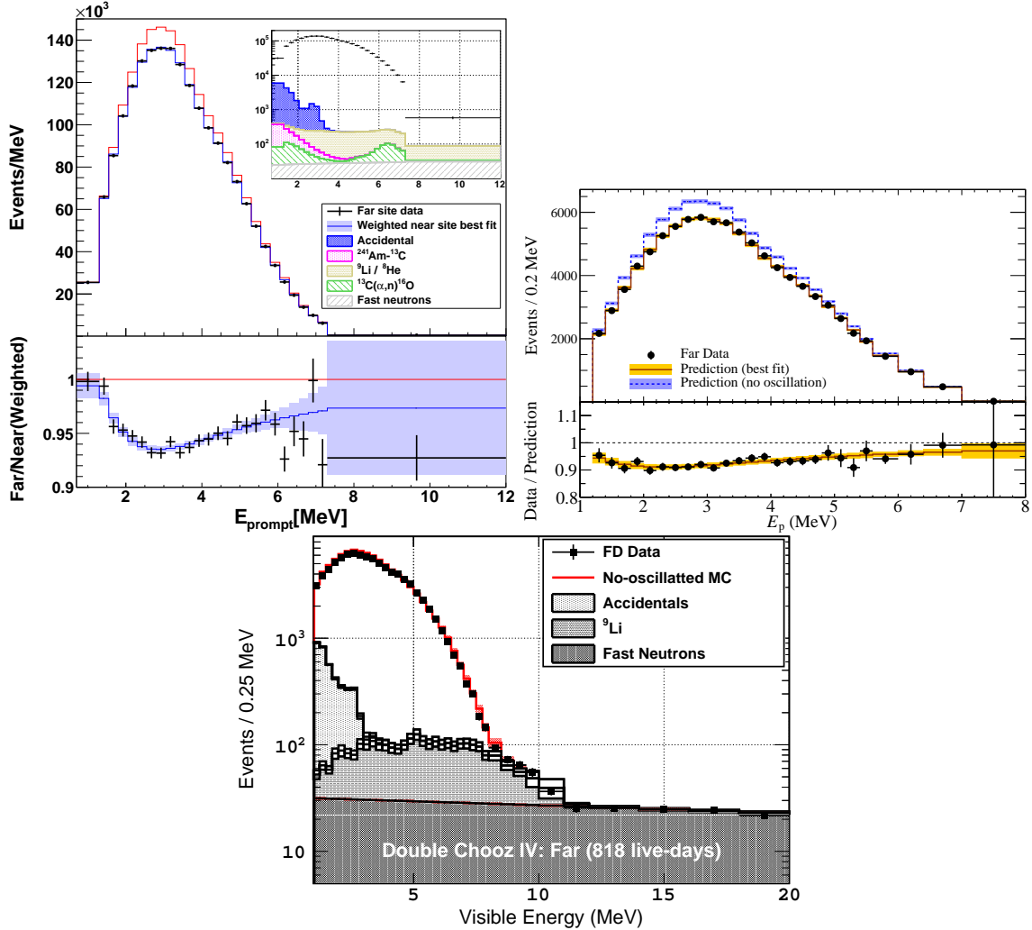
Figure 14.8: Energy spectra for prompt events at the far detectors for Daya Bay [141], RENO [142], and Double Chooz [143].
