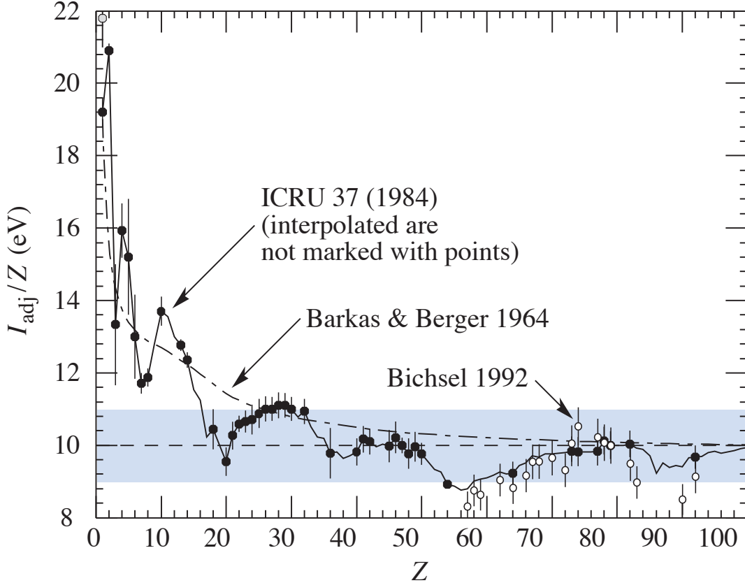
Figure 34.5: Mean excitation energies (divided by Z ) as adopted by the ICRU [12]. Those based on experimental measurements are shown by symbols with error flags; the interpolated values are simply joined. The grey point is for liquid \text{H}_2 ; the black point at 19.2 eV is for \text{H}_2 gas. The open circles show more recent determinations by Bichsel [13]. The dash-dotted curve is from the approximate formula of Barkas [14] used in early editions of this Review .
