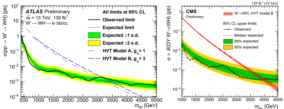
Figure 86.2: Upper limits on W' production cross section times branching fraction into a W and a SM Higgs boson decaying into heavy-flavor quarks, from ATLAS [49] (left) and CMS [46] (right).
