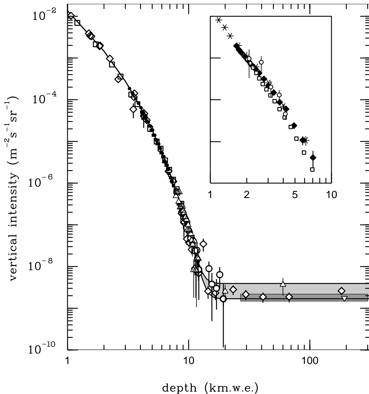
Figure 30.8: Vertical muon intensity vs depth (1 km.w.e. = 10^5 g \text{cm}^{-2} of standard rock). The experimental data are from: \diamond : the compilations of Crouch [84], \square : Baksan [85], \circ : LVD [86], \bullet : MACRO [87], \blacksquare : Frejus [88], and \triangle : SNO [89]. The shaded area at large depths represents neutrino-induced muons of energy above 2 GeV. The upper line is for horizontal neutrino-induced muons, the lower one for vertically upward muons. Darker shading shows the muon flux measured by the SuperKamiokande experiment. The inset shows the vertical intensity curve for water and ice published in Refs. [90–93]. Additional data extending to slant depths of 13 km are available in [94].
