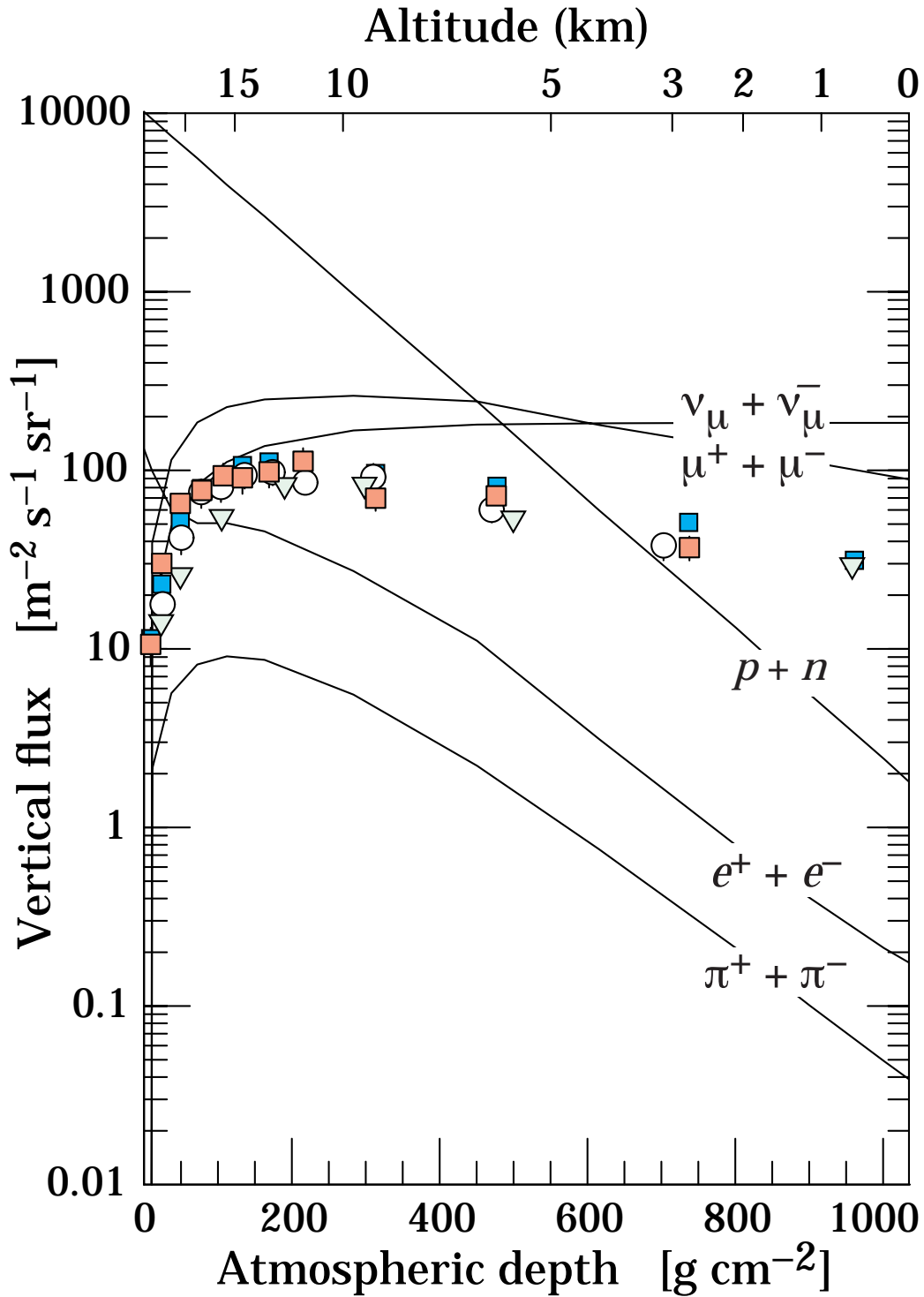
Figure 30.5: Vertical fluxes of cosmic rays in the atmosphere with E > 1 GeV estimated from the nucleon flux of Eq. (30.2). The experimental points show measurements of negative muons with E_{\mu} > 1 GeV [57–62].
