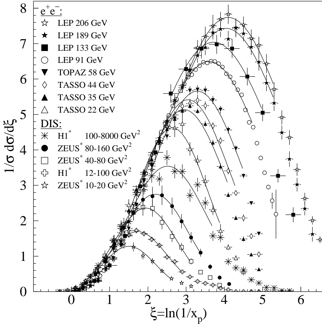
Figure 19.4: Distribution of the normalized fragmentation cross sections in \xi = \ln(1/x_p) at several CM energies ( e^+e^- ) [29, 30, 35–38, 57, 58, 75–78] and for intervals of Q^2 (DIS). At each energy only one representative measurement is displayed. For clarity some measurements at intermediate CM energies ( e^+e^- ) or Q^2 ranges (DIS) are not shown. The DIS measurements (*) have been scaled by a factor of 2 for direct comparability with the e^+e^- results. Fits of simple Gaussian functions are overlaid for illustration.
