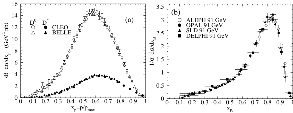
Figure 19.12: (a) Efficiency-corrected inclusive cross-section measurements for the production of D^0 and D^{*+} in e^+e^- measurements at \sqrt{s} \approx 10.6 GeV, excluding B decay products [292] [293]. (b) Measured e^+e^- fragmentation function of b quarks into B hadrons at \sqrt{s} \approx 91 GeV [296].
