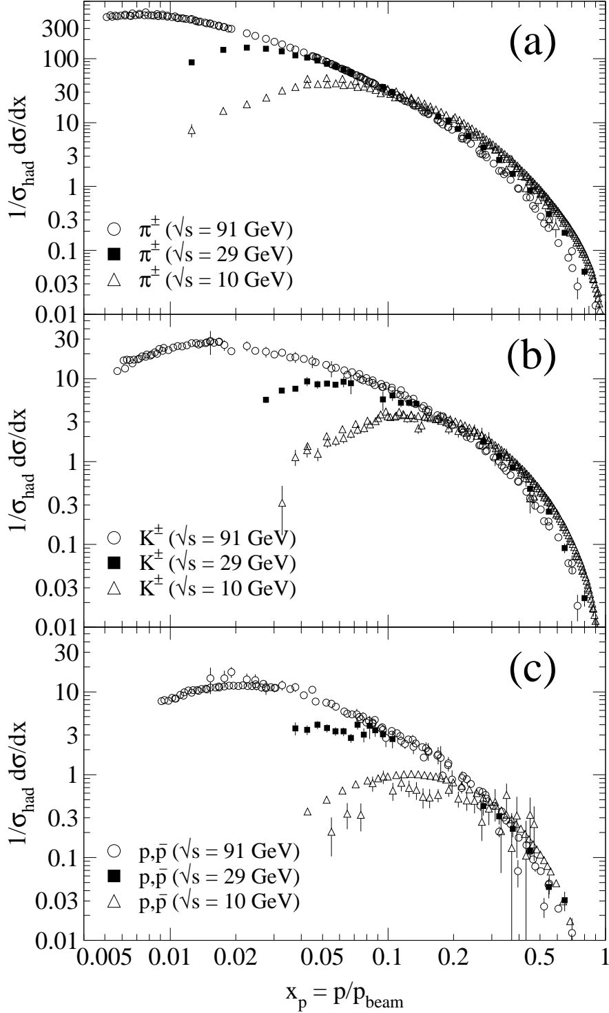
Figure 19.9: Scaled momentum spectra of (a) \pi^\pm , (b) K^\pm , and (c) p, \bar{p} at \sqrt{s} = 10, 29, and 91 GeV [43, 45, 85, 169, 194].
