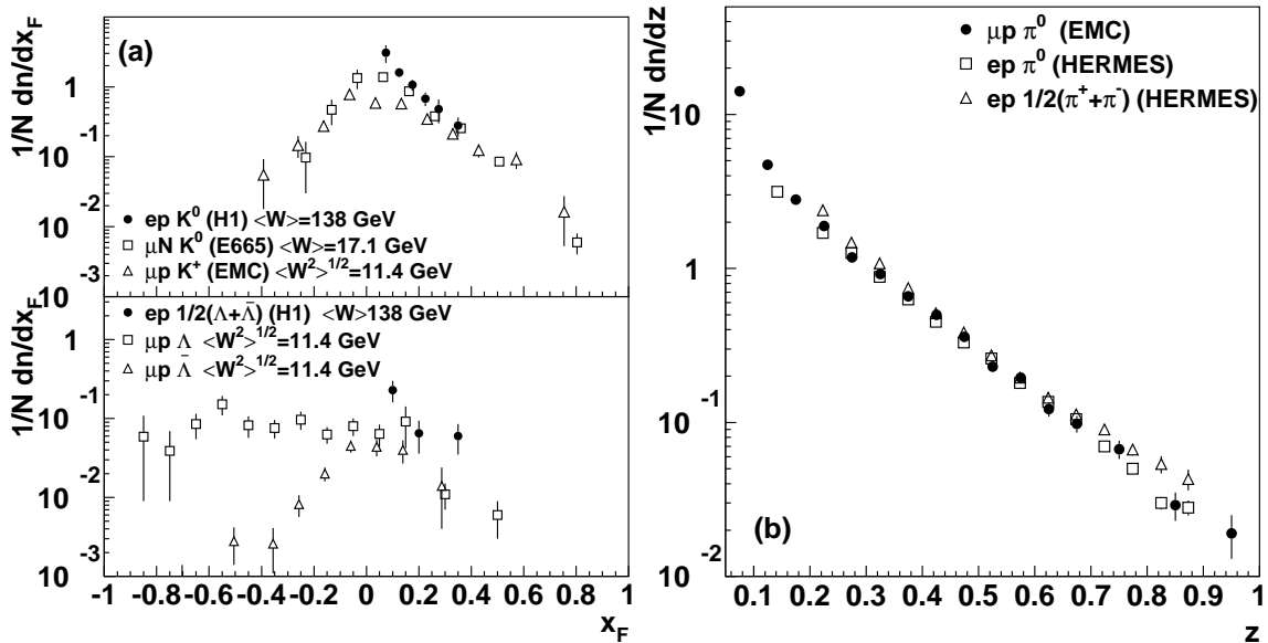
Figure 19.8: (a) 1/N \cdot dn/dx_F for identified strange particles in DIS at various values of W [174, 177, 182]. (b) 1/N \cdot dn/dz for measurements of pions in fixed-target DIS experiments [175, 178, 181].
