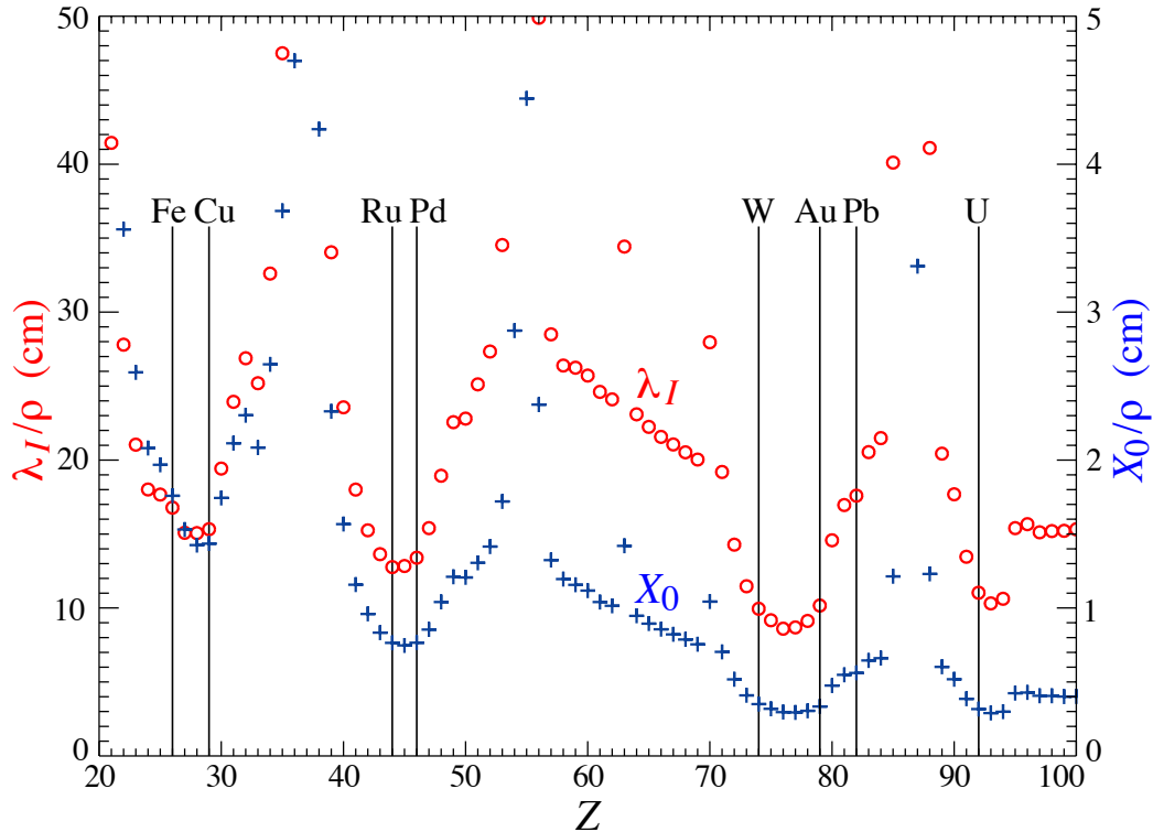
Figure 35.30: Nuclear interaction length \lambda_I/\rho (circles) and radiation length X_0/\rho (+’s) in cm for the chemical elements with Z > 20 and \lambda_I < 50 cm.
