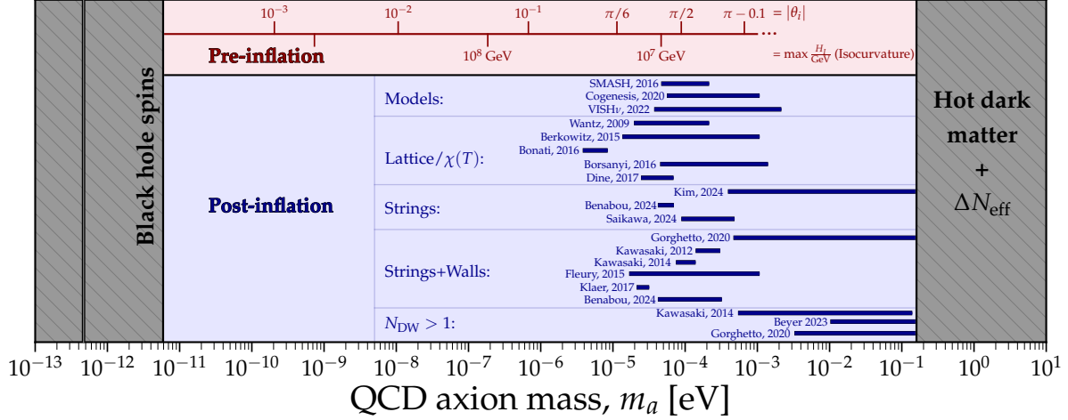
Figure 89.4: QCD axion mass predictions for obtaining the correct DM abundance assuming the PQ symmetry is and is not restored after inflation and, in the case the PQ symmetry is restored after inflation, depending on the domain wall number N . Figure from [63], includes data from refs. [24, 364–378]. The lower-end of the possible mass range is bounded by BH superradiance constraints and the theoretical requirement that f_a be below the Planck scale, while the upper end is bounded by the somewhat model-dependent NS cooling constraints (not shown), which exclude QCD axion masses above roughly \sim 15\text{--}30 meV, depending on the UV completion. At even higher masses there are strong constraints from the production of DM in the early universe, which behaves as hot DM and contributes to \Delta N_{\text{eff}} .
