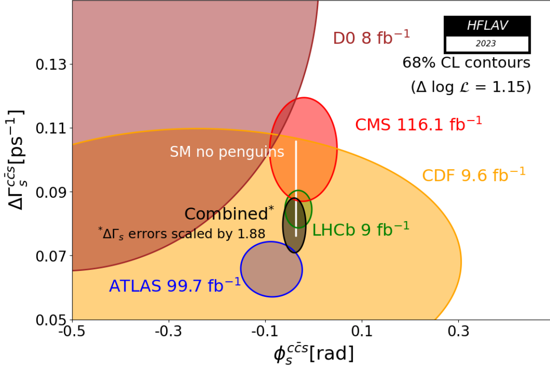
Figure 74.4: 68% CL contours in the (\phi_s^{ccs}, \Delta\Gamma_s) plane, showing all measurements from CDF [80], DØ [81], ATLAS [30,82], CMS [31,83] and LHCb [27,60,75,84–86,104,105] using B_s^0 decays governed by the b \rightarrow c\bar{c}s transition. Their average [8] is represented as the black ellipse, where the combined uncertainty on \Delta\Gamma_s has been multiplied by 1.88. The very thin white rectangle represents the Standard Model predictions of -2\beta_s [63,64] and \Delta\Gamma_s [7].
