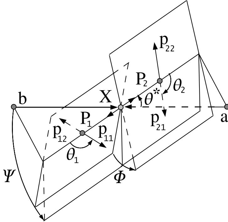
Figure 73.1: Definition of the production and helicity angles in the sequential process ab \rightarrow X \rightarrow P_1 P_2 \rightarrow (p_{11} p_{12})(p_{21} p_{22}) . The three helicity angles include \theta_1 and \theta_2 , defined in the rest frame of the two daughters P_1 and P_2 , and \Phi , defined in the X frame as the angle between the two decay planes. The two production angles \theta^* and \Psi are defined in the X frame, where \Psi is the angle between the production plane and the average of the two decay planes.
