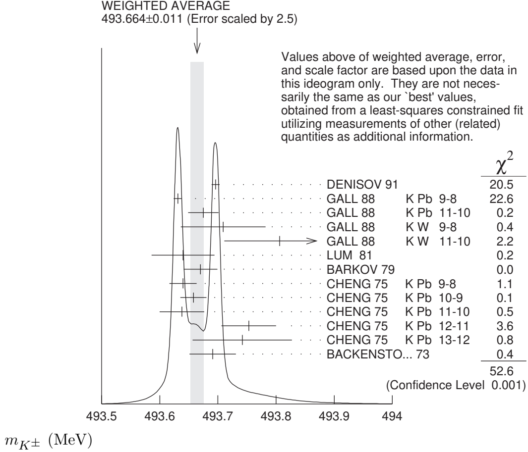
Figure 1: Ideogram of m_{K^\pm} mass measurements. GALL 88 and CHENG 75 measurements are shown separately for each transition they measured.
