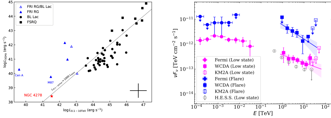
Figure 30.13: Upper panels: radio luminosity vs. TeV luminosity involving the detection of NGC 4278 (left), Gamma-ray SED of M87 for the low state and flare state (right)
