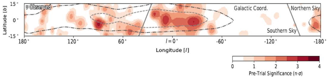
Figure 30.17: The Milky Way plane in neutrinos (Galactic coordinates, with the origin being at the Galactic Center). Shown is the pre-trial significance of the IceCube observations using a cascade neutrino event sample, calculated from an all-sky scan for point-like sources [311]. Contours indicate the regions that contain 20% and 50% of the predicted diffuse neutrino emission according to an extrapolation of Fermi-LAT results. Gray lines indicate the Northern-Southern sky horizon line.
