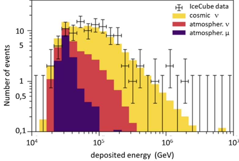
Figure 30.16: Measured (data points) and expected (histograms) distributions of the deposited energy measured in the IceCube detector for events passing the HESE selection, which strongly suppresses down-going atmospheric neutrinos by vetoing accompanying muons. The cosmic neutrino flux has been assumed to follow an unbroken power law in E_\nu . Its normalization and spectral index, as well as the normalizations of the conventional and prompt atmospheric neutrino and the atmospheric muon contributions were fitted to the data, where only the region above 60 TeV was used to constrain the cosmic neutrino flux.
