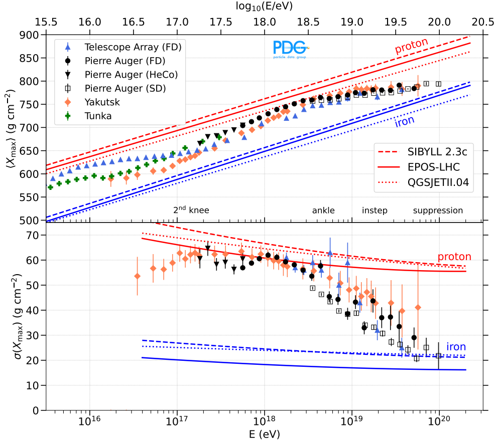
Figure 30.8: Measurements of the mean depth of shower maximum, \langle X_{\max} \rangle (top), and its standard deviation, \sigma(X_{\max}) (bottom), obtained by the Telescope Array [169,170]; Pierre Auger Observatory [164, 171, 172]; Yakutsk [146]; and Tunka [144] detectors. These measurements are compared to model predictions for proton and iron primaries using hadronic interaction models SIBYLL2.3c [173], EPOS-LHC [136], and QGSJET-II.04 [135]. The detection techniques include fluorescence (FD and HeCo), Cherenkov light detection (Yakutsk, Tunka, and Telescope Array below \simeq 1 , EeV), and surface array measurements (Auger SD using deep-learning techniques). For a comprehensive compilation that includes experiments using radio detection techniques, see [167] and [174].
