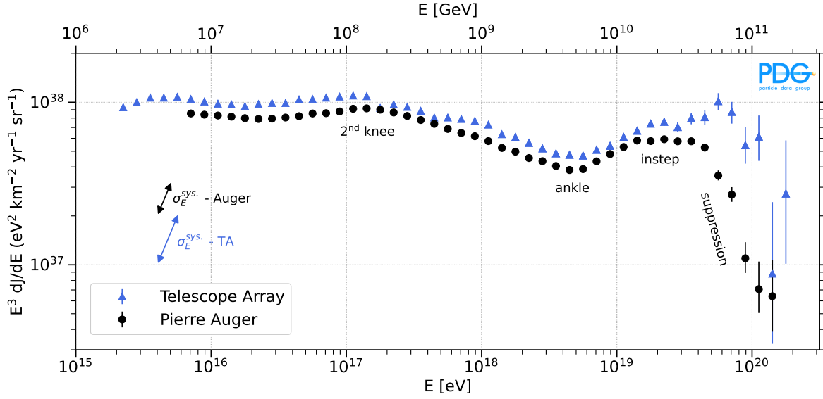
Figure 30.7: Measurements of the all-particle CR flux from Telescope Array (TA) [165] (blue triangles) and the Pierre Auger Observatory [33, 166] (black circles). The direction and magnitude of the systematic uncertainty on the flux due to the energy scale ( \sigma_E^{\text{sys}} ) for TA and Auger is indicated by the corresponding arrows. For a comprehensive compilation of measurements see [167].
