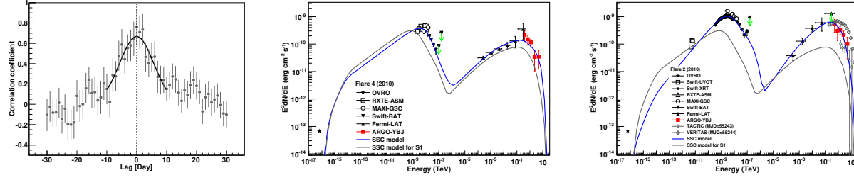
Figure 30.12: The multi wavelength analysis of Mrk 421 involving measurements over wide energy range from radio to TeV \gamma -ray during 4.5 years when ARGO-YBJ and LAT were operated [269]. The discrete correlation function between the light curves in X-ray band and TeV \gamma -ray band is calculated and clearly shows no time lag between emissions in the two bands [269] (left panel). The SED significantly changes from steady states (gray solid lines in middle and right panels) to flaring states depending on the strength of flares. Comparing a small flare in the middle panel and a larger one in right panel, the later has harder SED in VHE band [267].
