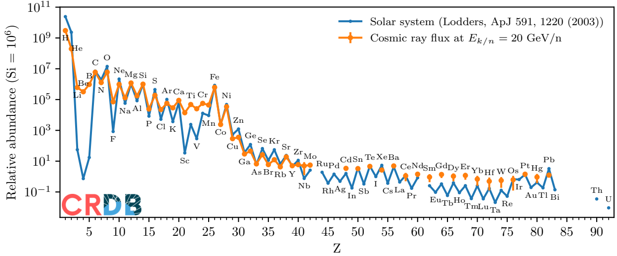
Figure 30.2: CR abundances compared with solar system ones [65]. Modified from [37].
