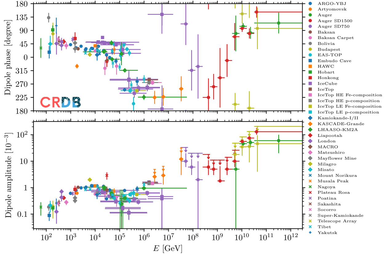
Figure 30.5: Phase and amplitude of the dipole anisotropy in CRs. Modified from Ref. [37].
