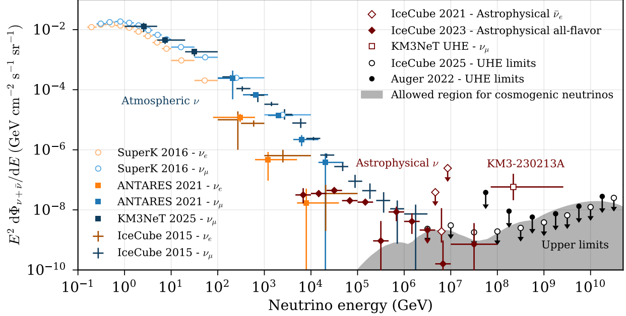
Figure 30.15: Measured energy spectra of atmospheric and cosmic diffuse neutrino fluxes. Experimental limits at highest energy are compared to model predictions for cosmogenic neutrinos [192]. All fluxes are normalized to one flavor ( \nu + \bar{\nu} ), assuming a ratio \bar{\nu} : \nu = 1 and, for cosmic neutrinos, a ratio \nu_e : \nu_\mu : \nu_\tau = 1 : 1 : 1 at Earth. Data sources: SuperK 2016 [290]; ANTARES 2021 [291]; KM3NeT 2025 \nu_\mu [292]; IceCube 2015 \nu_e [293]; IceCube 2015 \nu_\mu [294]; IceCube 2021 astrophysical \bar{\nu}_e ( \nu + \bar{\nu} flux derived from a single candidate event for the Glashow resonance) [295]; IceCube 2023 astrophysical all flavor [43], KM3NeT-UHE \nu_\mu [187]. The limits at the highest energies are taken from [296] (IceCube) and [297] (Auger). They are shown in the energy bins used for the corresponding analyses and have been adjusted to bin widths of one decade. The region allowed for the expected cosmogenic neutrino fluxes is taken from [298] (see also Fig. 36.10).
