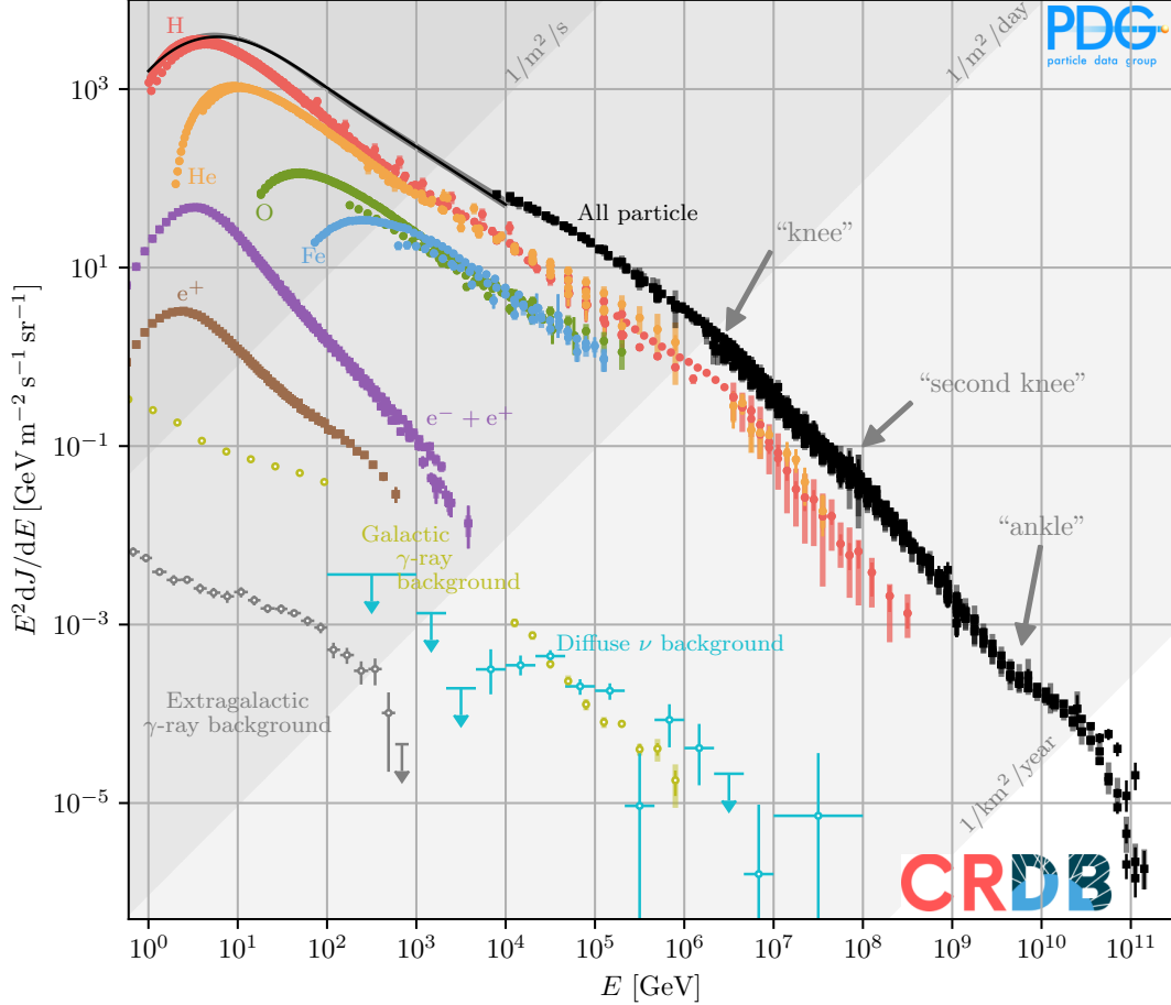
Figure 30.1: The spectrum of cosmic rays (CRs). Shown are measurements of the intensity of charged and neutral CRs, multiplied by kinetic energy squared. The data for the charged CRs [5–36] have been extracted from the Cosmic Ray Database (CRDB) [37] and we also include preliminary LHAASO proton data [38]. Below 10^4 GeV, the all-particle spectrum is the sum of spline fits of the most important nuclear species. The diffuse \gamma -ray fluxes have been extracted from Refs. [39–42], measurements of the diffuse neutrino background from Ref. [43]. Energy-integrated intensities are indicated by the various diagonal lines.
