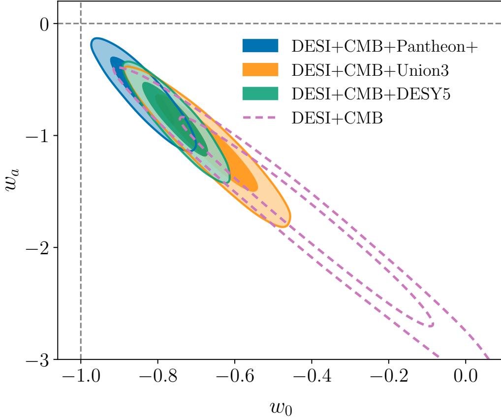
Figure 28.2: Constraints on parameters of the w_0w_a CDM dark energy model from combinations of CMB, BAO, and supernova (SN) data, taken from Ref. [37]. Dashed contours show 68% and 95% confidence intervals on w_0 and w_a inferred from DESI DR2 BAO measurements and Planck 2018 CMB anisotropy data. Filled contours show the impact of adding SN data from the DES Y5 compilation (green), the Pantheon+ compilation (blue), or the Union3 compilation (orange). Dashed gray lines mark the \Lambda CDM values of w_0 = -1 , w_a = 0 .
