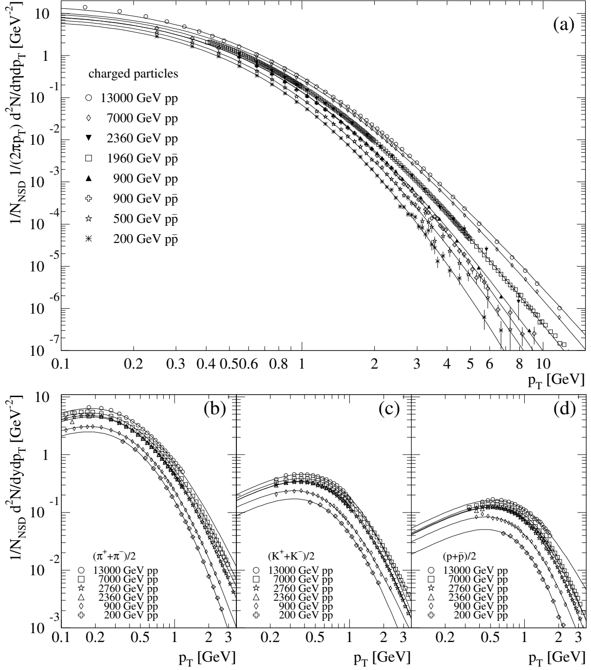
Figure 19.11: (a) Selection of inclusive charged-particle transverse momentum spectra [114, 117, 119, 121, 161, 212, 213], normalized to the non-single diffractive cross section (NSD). (b)-(d) Selection of identified charged-particle transverse momentum spectra [214–219] normalized to the NSD cross section. All spectra are scaled to the NSD cross-section using measurements of total, inelastic, elastic, single, or non-single diffractive cross sections from [220–224, 224–226]. The overall normalization uncertainty of about 3% is not shown. Superimposed are fits of the Tsallis distribution in Eq. (19.13).
