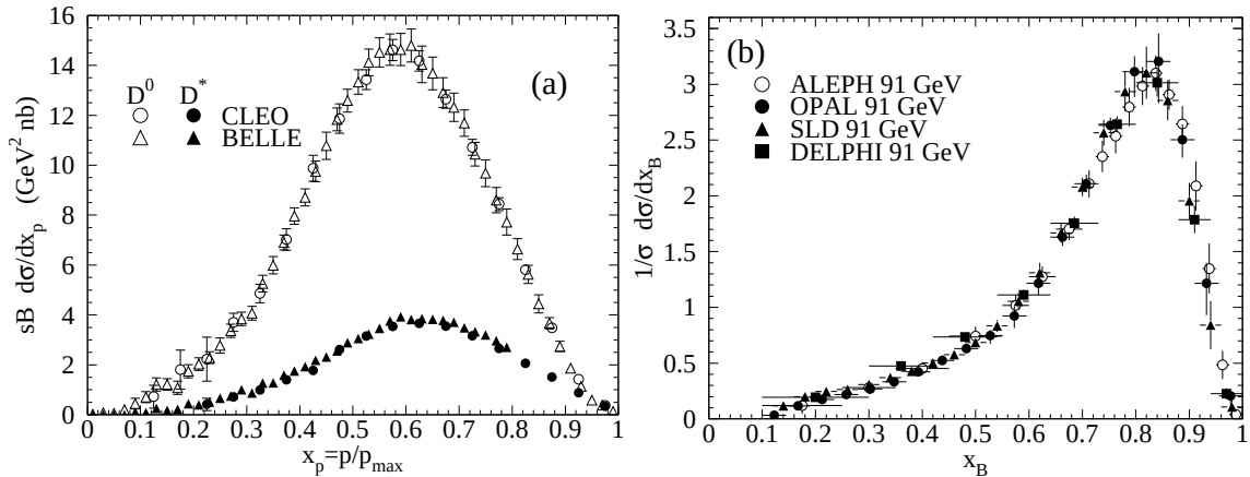
Figure 19.12: (a) Efficiency-corrected inclusive cross-section measurements for the production of D^0 and D^{*+} in e^+e^- measurements at \sqrt{s} \approx 10.6 GeV, excluding B decay products [283] [284]. (b) Measured e^+e^- fragmentation function of b quarks into B hadrons at \sqrt{s} \approx 91 GeV [285].
