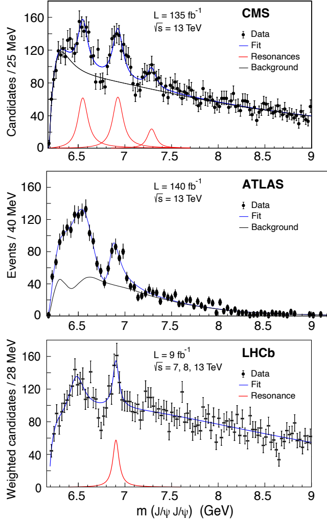
Figure 77.4: J/\psi(1S) -pair invariant mass distributions measured by the LHCb [79] (bottom), ATLAS [80] (middle), and CMS [81] (top) experiments.
