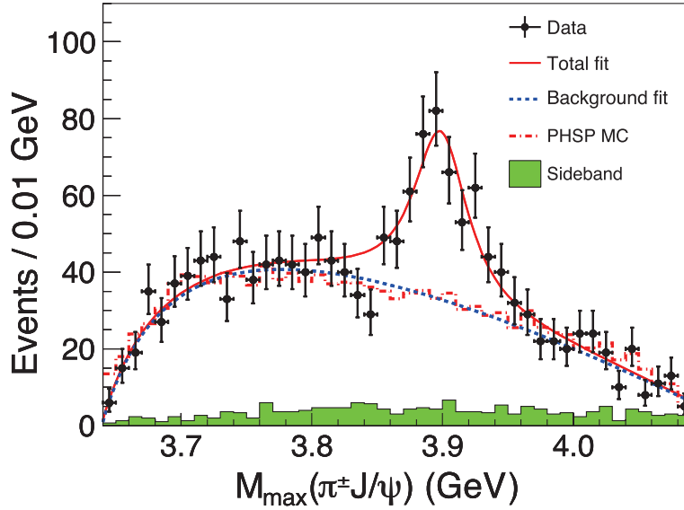
Figure 77.5: The \pi^\pm J/\psi(1S) invariant mass distribution from BESIII [97] e^+e^- collision data taken at a center-of-mass energy near 4260 MeV.
