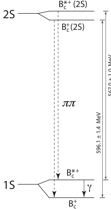
Figure 77.3: Diagram showing the decays mentioned in the text.
