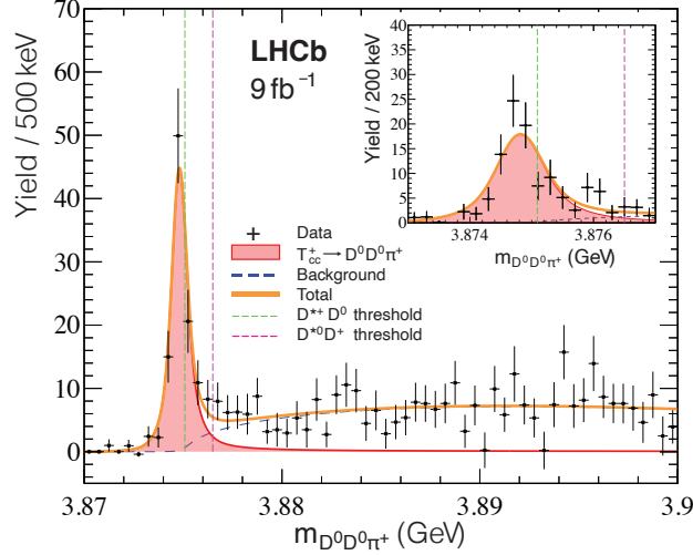
Figure 77.6: The D^0 D^0 \pi^+ invariant mass distribution from LHCb [109, 110].
