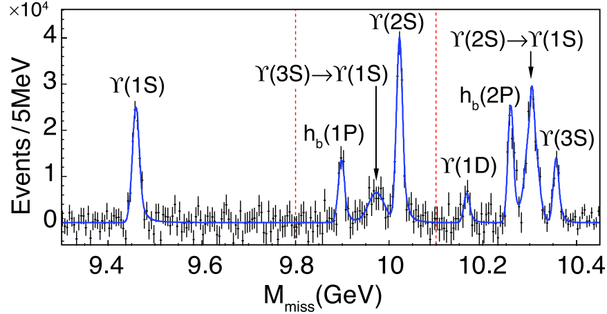
Figure 77.1: From Belle [26], the mass recoiling against \pi^+\pi^- pairs, M_{\text{miss}} , in e^+e^- collision data taken near the peak of the \Upsilon(10860) . The smooth combinatorial and K_S^0 \rightarrow \pi^+\pi^- background contributions have been subtracted. The fit to the various labeled signal contributions is overlaid (curve). The fit is performed separately in three regions with boundaries indicated by the vertical dashed lines.
