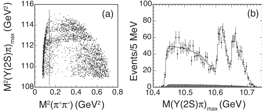
Figure 77.7: From Belle [111] e^+e^- collision data taken near the peak of the \Upsilon(10860) for events with a \pi^+\pi^- -missing mass consistent with an \Upsilon(2S) \rightarrow \mu^+\mu^- , (a) the maximum of the two possible single \pi^\pm -missing-mass-squared combinations vs. the \pi^+\pi^- -mass-squared; and (b) projection of the maximum of the two possible single \pi^\pm -missing-mass combinations overlaid with a fit ( curve ). Events to the left of the vertical line in (a) are excluded from the amplitude analysis. The hatched histogram in (b) corresponds to the combinatorial background. The two horizontal stripes in (a) and two peaks in (b) correspond to the two T_{b\bar{b}} states.
