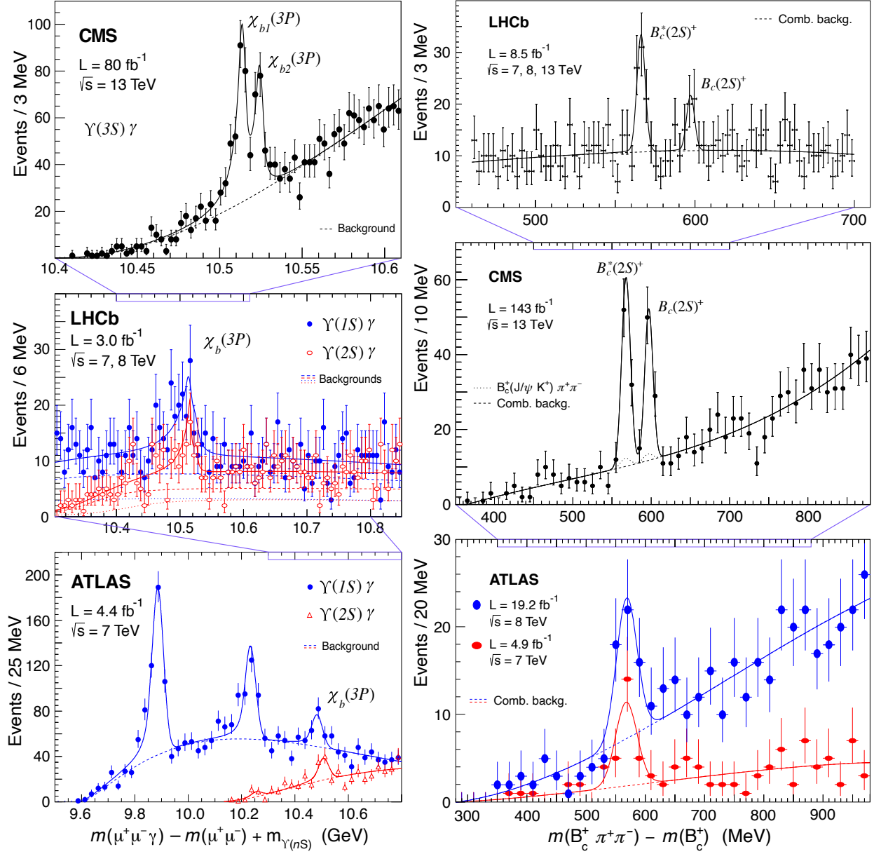
Figure 77.2: (Left Column) Invariant mass distributions measured by the ATLAS [29] (bottom), LHCb [31] (middle) and CMS [32] (top) experiments in their searches for the \chi_b(3P) states through their radiative decays to one of the S-wave bottomonia. (Right Column) Invariant mass distributions measured by the ATLAS [33] (bottom), CMS [34] (middle) and LHCb [35] (top) experiments in their searches for B_c^\pm excited states decaying to the B_c^\pm ground state with the emission of two charged pions.
