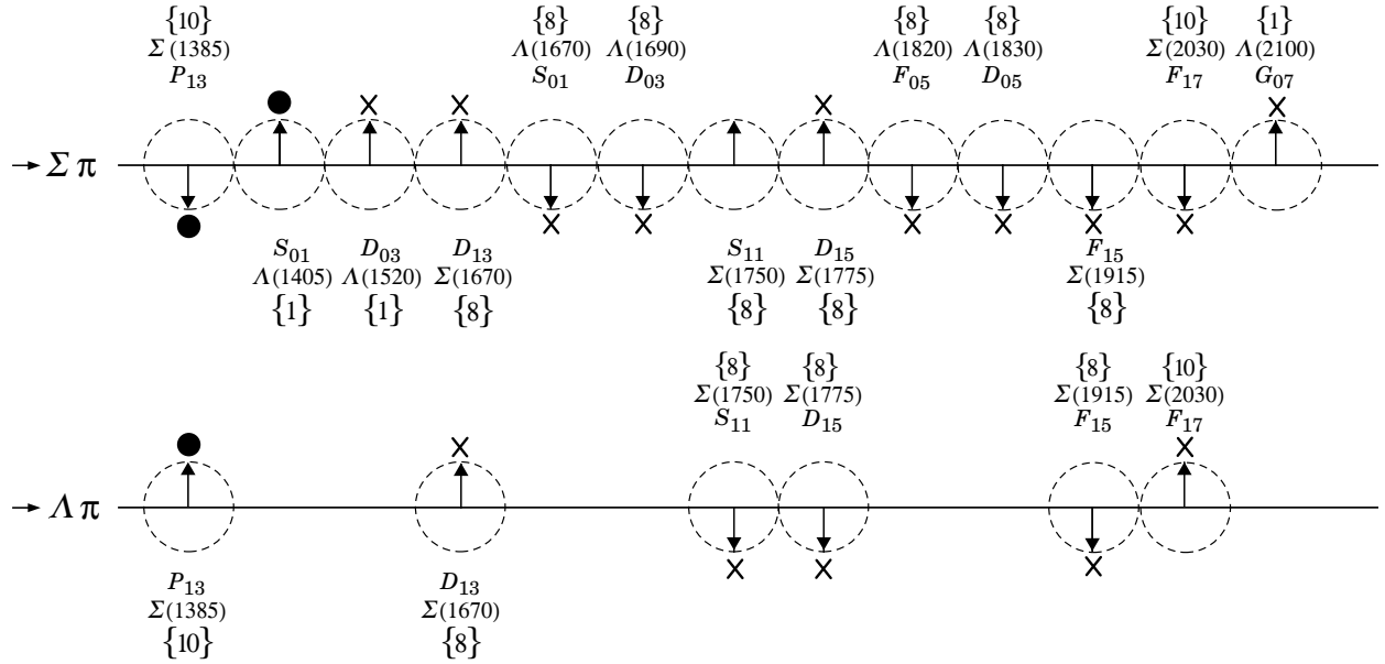
Figure 81.1: The signs of the imaginary parts of resonating amplitudes in the \bar{K}N \rightarrow \Lambda\pi and \Sigma\pi channels. The signs of the \Sigma(1385) and \Lambda(1405) , marked with a \bullet , are set by convention, and then the others are determined relative to them. The signs required by the SU(3) assignments of the resonances are shown with an arrow, and the experimentally determined signs are shown with an \times .
