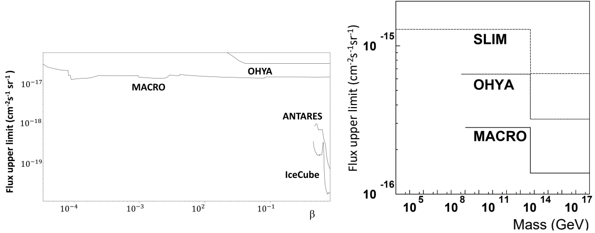
Figure 94.1: Left: upper flux limits for GUT monopoles as a function of \beta . Right: upper flux limits for monopoles as a function of monopole mass for \beta > 0.05 .
