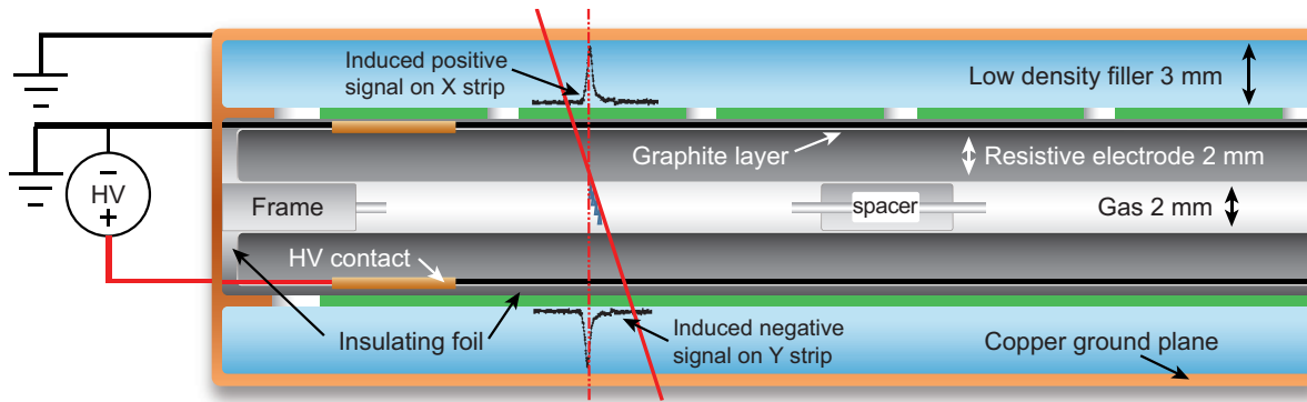
Figure 35.19: Schematic cross section of a generic single gap RPC. The thickness values shown are given just as an example.
