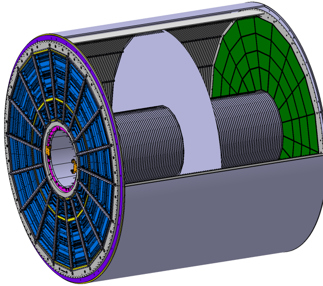
Figure 35.14: Schematic view of the ALICE TPC [195, 196]. The drift volume with 5 m diameter is divided into two halves, each providing 2.5 m drift length. The amplification stage has recently been upgraded from wire planes to GEMs.
