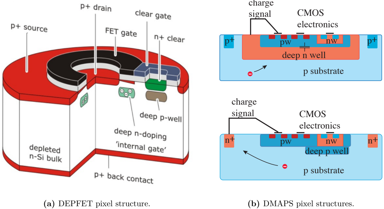
Figure 35.28: Partially (a) and fully (b) monolithic pixels: (a) A circular DEPFET pixel structure with an embedded pMOSFET transistor; source and drain are p implants (red), gate metal (black), oxide (grey), deep- n internal gate (light green), other metal (blue), clear contact (green), and deep p -well (brown). (b) Depleted MAPS with joint sensing and electronics volumes: (top) charge collection by a large-electrode which houses the electronics in a deep- n well; (bottom) charge collection by a small electrode set aside from the electronics area.
