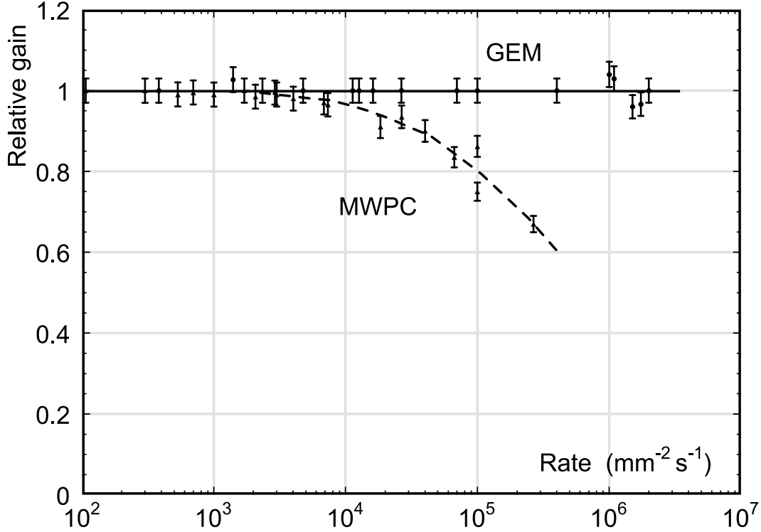
Figure 35.12: Normalized gas gain as a function of particle rate for MWPC [174] and GEM [175].
