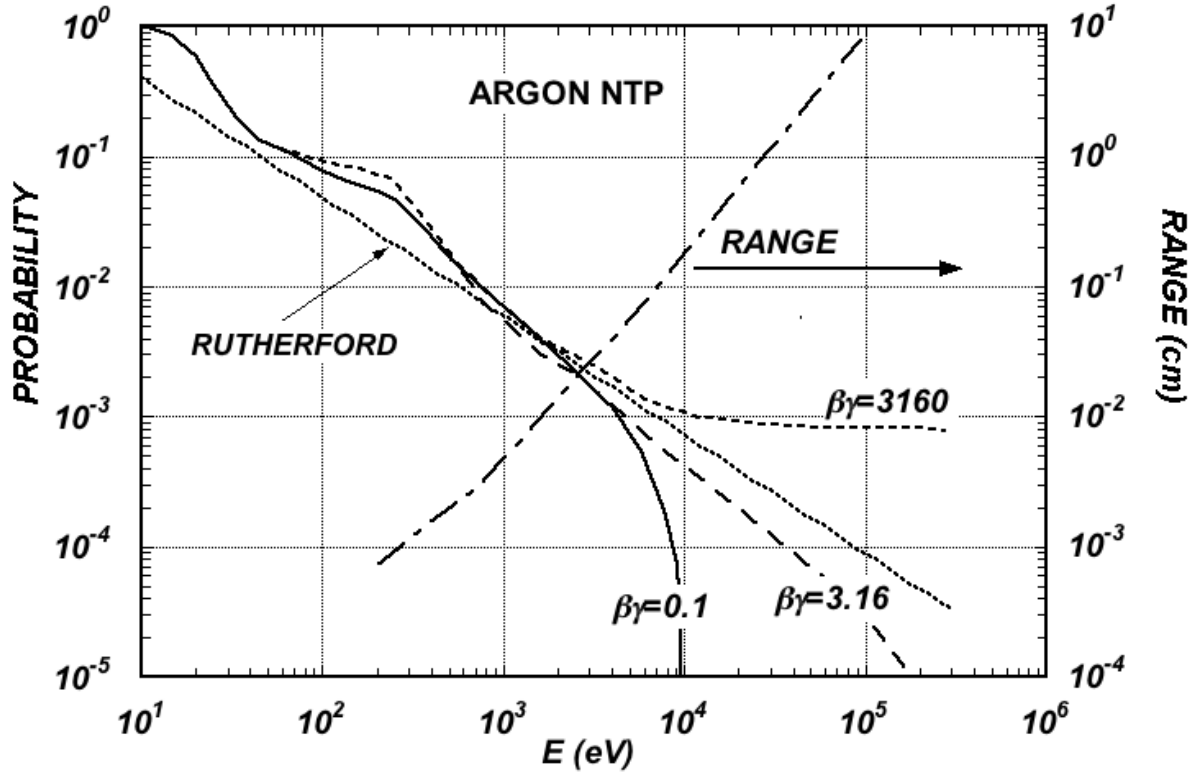
Figure 35.4: Probability of single collisions in which released electrons have an energy E or larger (left scale) and practical range of electrons in Ar at NTP (dot-dashed curve, right scale) [128].
