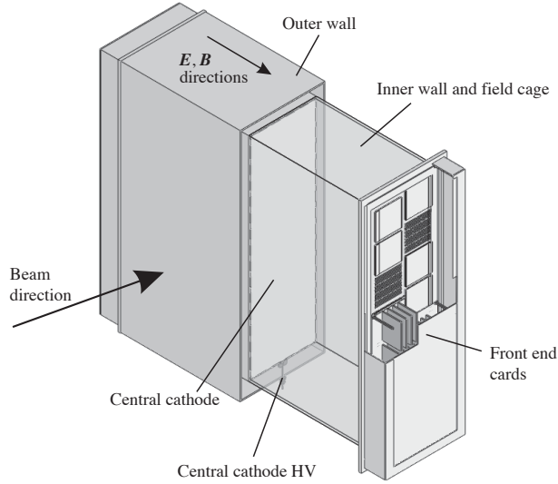
Figure 35.15: One of the 3 TPC modules for the near detector of the T2K experiment [197]. The size is 2 \times 2 \times 0.8 \text{ m}^3 . Micromegas devices are used for gas amplification and readout.
