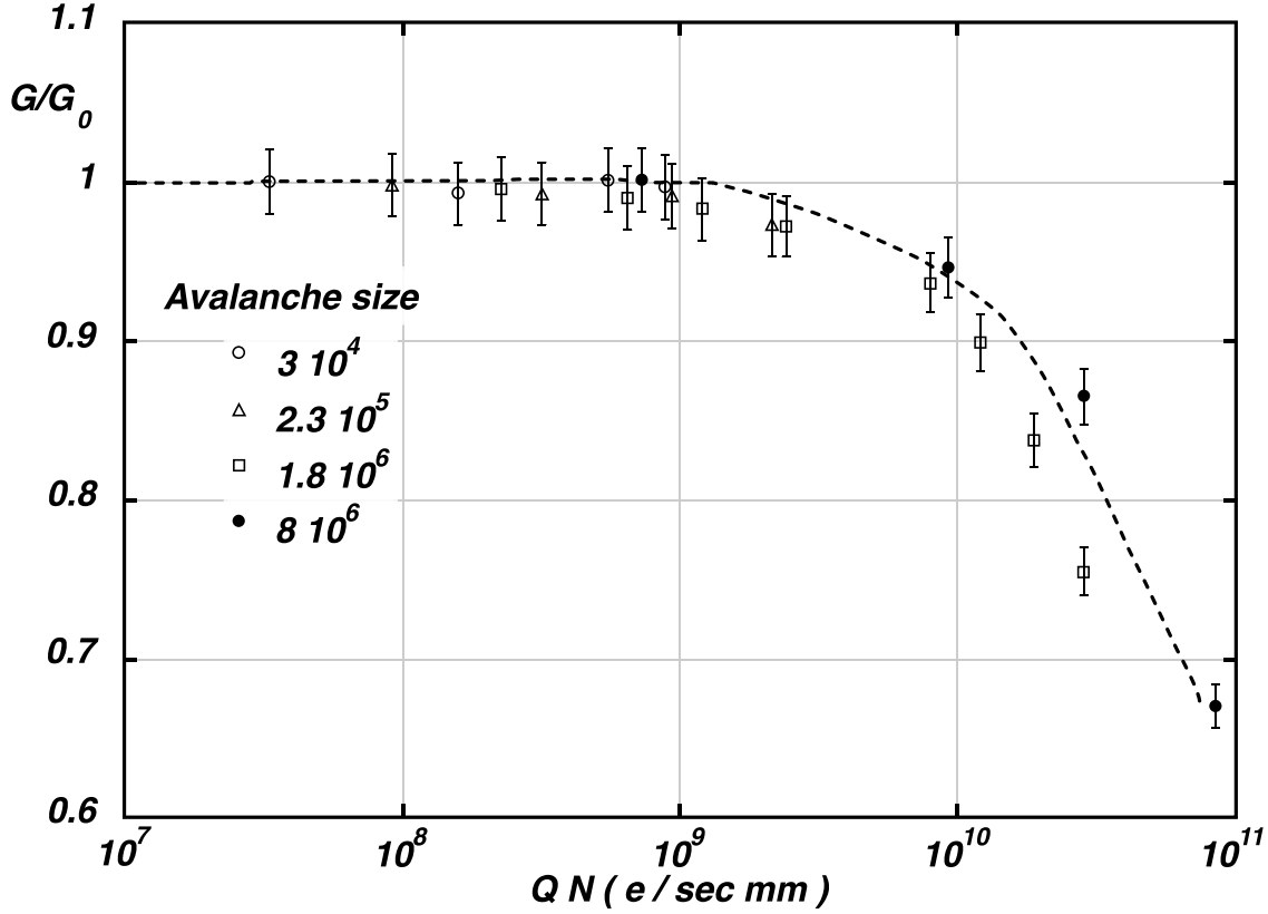
Figure 35.9: Charge rate dependence of normalized gas gain G/G_0 (relative to zero counting rate) in proportional thin-wire detectors [161]. Q is the total charge in a single avalanche; N is the particle rate per wire length.
