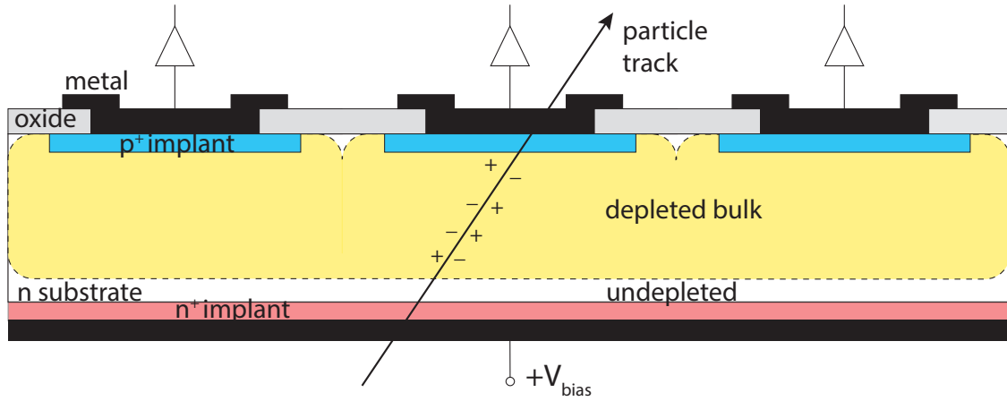
Figure 35.24: Reverse-bias junction detector with planar readout electrodes at the top in a standard sensor configuration ( p^+ -in- n ): lightly doped n -type substrate with p^+ implants forming the diode junction at the top side. Electrons move to the bottom electrode and holes to the top. Both movements contribute to the (induced) signal at the top electrodes with amounts as specified by the weighting field (see Sec. 35.8.1.2). The n^+ implant at the bottom side forms an ohmic contact between bulk and metal.
