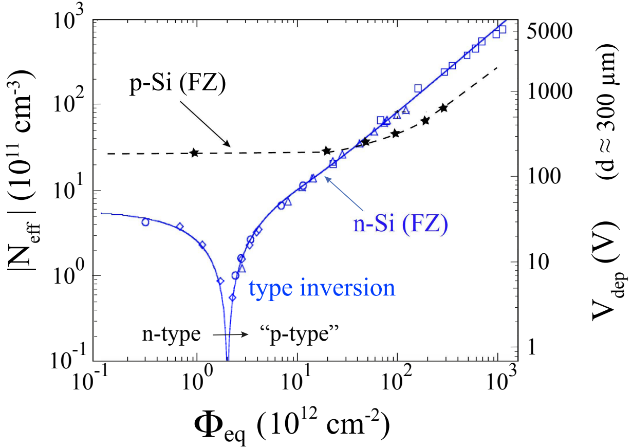
Figure 35.31: Effective space charge concentration N_{\text{eff}} (left axis) and required voltage for full depletion V_{\text{dep}} (right axis) of approximately 300 \mu\text{m} thick Si sensors as a function of neutron-equivalent radiation fluence for typical n -type (blue) and p -type (black) silicon float zone (FZ) material before annealing. While initial n -type Si inverts to effectively p -type Si, this is not observed for initial p -type silicon. Bias voltage supply for large systems is usually limited to less than 600–1000 V. Figure adapted using [429, 430] and [431].
