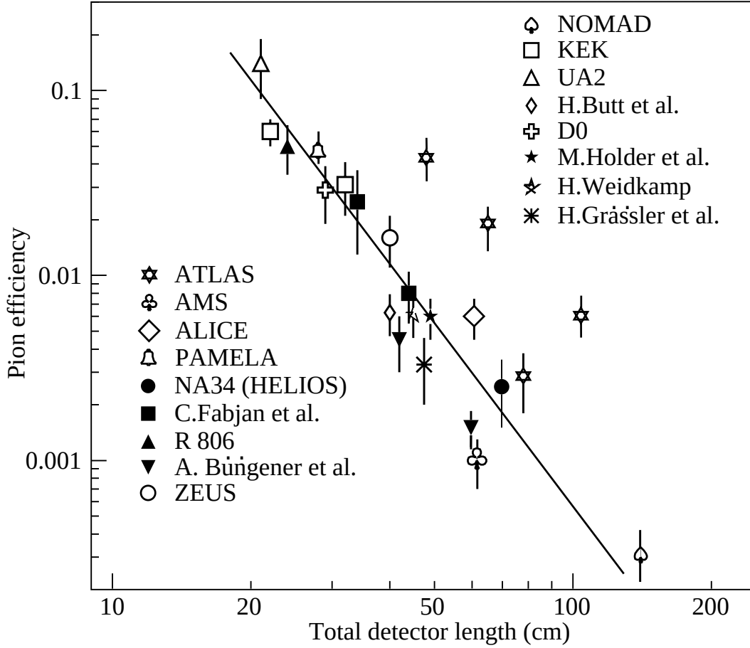
Figure 35.18: Pion efficiency measured (or predicted) for different TRDs as a function of the detector length for a fixed electron efficiency of 90%. The plot is based on the table given in [205]. Results from more recent detectors are added from [206, 210–212, 219].
