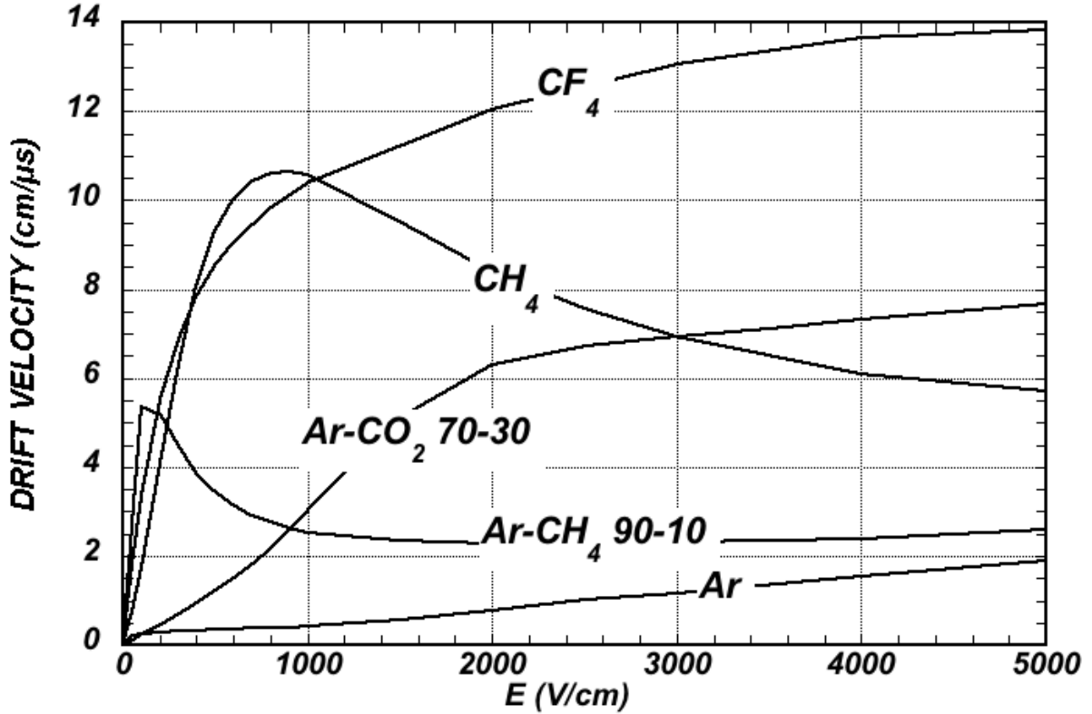
Figure 35.5: Computed electron drift velocity as a function of electric field in several gases at NTP and B = 0 [131, 132].
