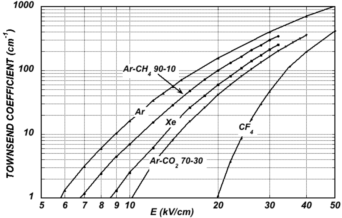
Figure 35.7: Computed first Townsend coefficient \alpha as a function of the electric field in several gases at NTP [131, 132].
