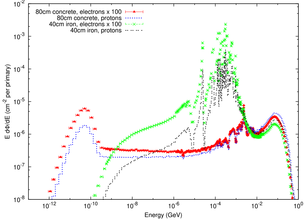
Figure 37.3: Neutron energy spectra calculated with the FLUKA code [9,10] from 25 GeV proton and electron beams on a thick copper target. Spectra are evaluated at 90^\circ to the beam direction behind 80 cm of concrete or 40 cm of iron. All spectra are normalized per beam particle. For better visualization, spectra for electron beam are multiplied by a factor of 100.
