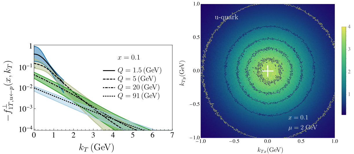
Figure 18.9: (Left) Sivers function in the momentum space for u quark [261] at x = 0.1 as a function of transverse momentum k_T for different values of Q . The bands are 68%CI. (Right) Momentum space density function as defined in [261] for the unpolarized u quark in a proton totally polarized in the y direction. The white cross indicates the origin with respect to which a shift of the distribution along the x -direction due to the Sivers function can be seen. The width of the patterns in the plot roughly indicates the uncertainty of the extraction.
