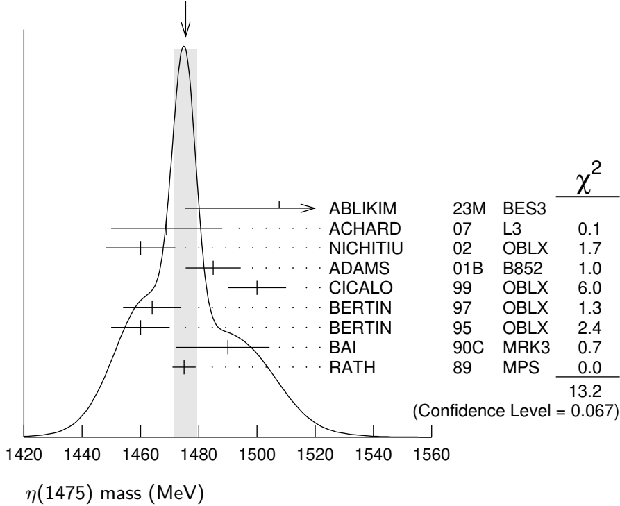
WEIGHTED AVERAGE 1476±4 (Error scaled by 1.4)
