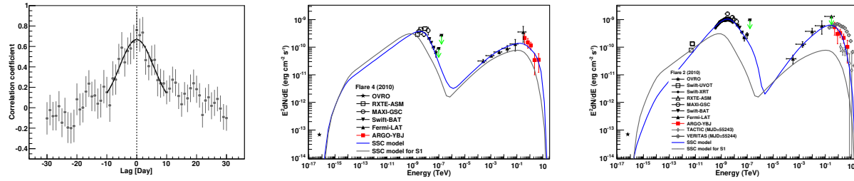
Figure 30.12: The multi wavelength analysis of Mrk 421 involving measurements over wide energy range from radio to TeV \gamma -ray during 4.5 years when ARGO-YBJ and LAT were operated [283]. The discrete correlation function between the light curves in X-ray band and TeV \gamma -ray band is calculated and clearly shows no time lag between emissions in the two bands [283] (left panel). The SED significantly changes from steady states (gray solid lines in middle and right panels) to flaring states depending on the strength of flares. Comparing a small flare in the middle panel and a larger one in right panel, the later has harder SED in VHE band [281].
