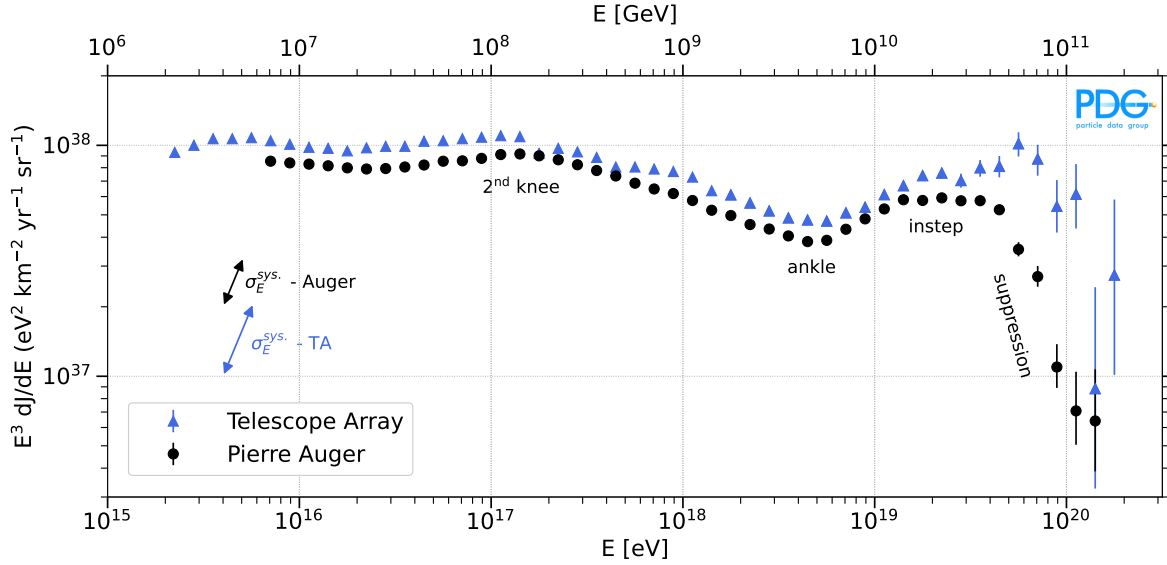
Figure 30.7: Measurements of the all-particle CR flux from Telescope Array (TA) [169] (blue triangles) and the Pierre Auger Observatory [33, 170] (black circles). The direction and magnitude of the systematic uncertainty on the flux due to the energy scale ( \sigma_E^{\text{sys}} ) for TA and Auger is indicated by the corresponding arrows. For a comprehensive compilation of measurements see [171].
