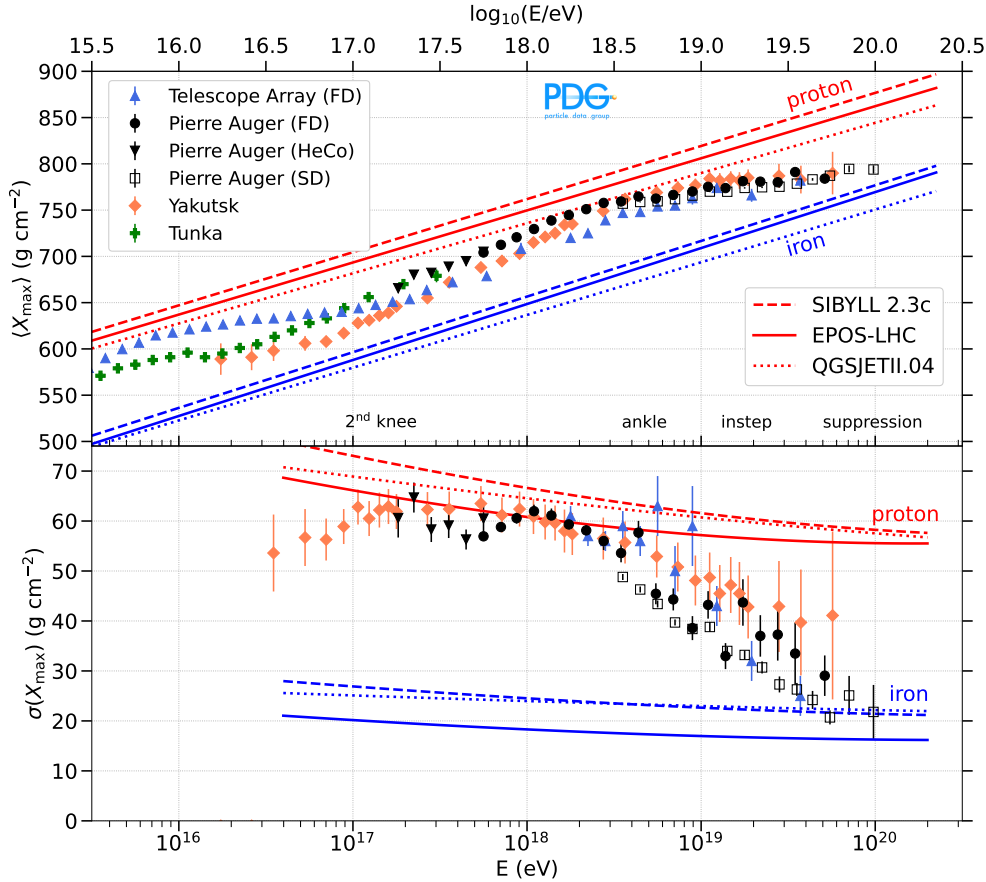
Figure 30.8: Measurements of the mean depth of shower maximum, \langle X_{\max} \rangle (top), and its standard deviation, \sigma(X_{\max}) (bottom), obtained by the Telescope Array [173, 174]; Pierre Auger Observatory [168, 175, 176]; Yakutsk [149]; and Tunka [147] detectors. These measurements are compared to model predictions for proton and iron primaries using hadronic interaction models SIBYLL2.3c [177], EPOS-LHC [139], and QGSJET-II.04 [138]. The detection techniques include fluorescence (FD and HeCo), Cherenkov light detection (Yakutsk, Tunka, and Telescope Array below \simeq 1 , EeV), and surface array measurements (Auger SD using deep-learning techniques). For a comprehensive compilation that includes experiments using radio detection techniques, see [171] and [178].
