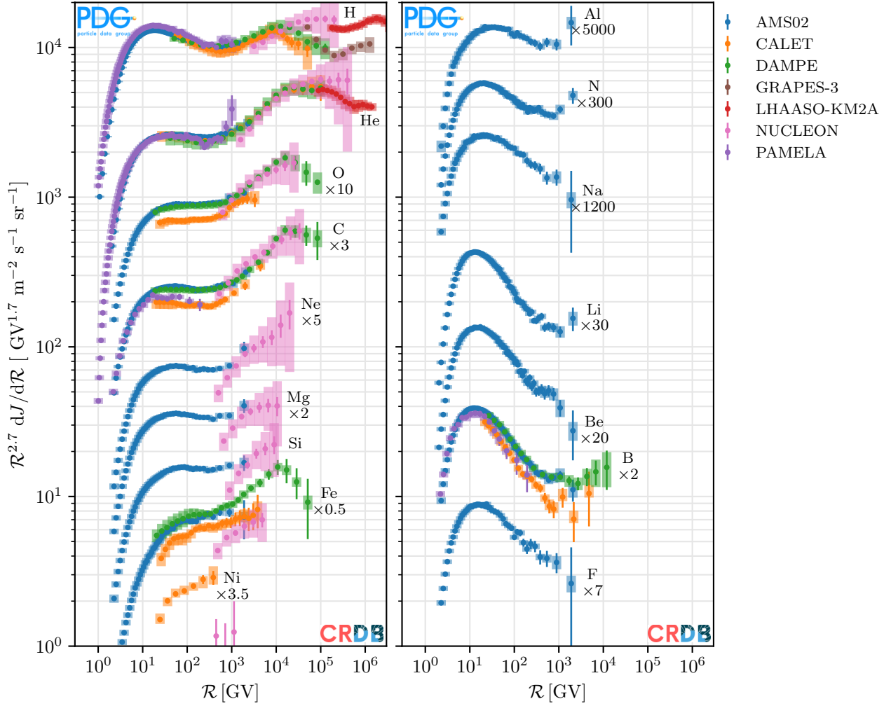
Figure 30.3: Rigidity spectra for a selection of CR nuclei. Primary species are shown in the left panel, (mostly) secondary species in the right panel. The error bars denote the statistical uncertainties, the shaded bars represent the systematic uncertainties. The spectra have been shifted and multiplied by \mathcal{R}^{2.7} to better bring out spectral features. Here, we have constrained ourselves to data from space-borne experiments of the last ten years, that is AMS-02 [12, 19, 86–89], CALET [14, 20, 90–92], DAMPE [11, 17, 37, 93], NUCLEON [9] and PAMELA [6, 94], but also included the ground-based GRAPES-3 [36] experiment and LHAASO data [39, 40]. Data have been extracted from [38].
