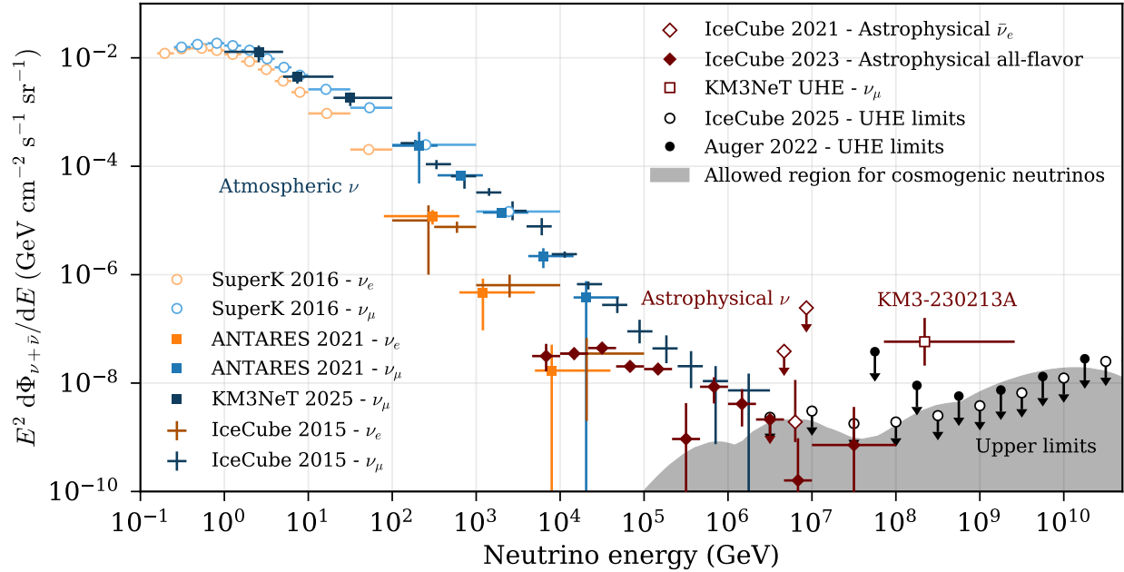
Figure 30.15: Measured energy spectra of atmospheric and cosmic diffuse neutrino fluxes. Experimental limits at highest energy are compared to model predictions for cosmogenic neutrinos [198]. All fluxes are normalized to one flavor ( \nu + \bar{\nu} ), assuming a ratio \bar{\nu} : \nu = 1 and, for cosmic neutrinos, a ratio \nu_e : \nu_\mu : \nu_\tau = 1 : 1 : 1 at Earth [305]; ANTARES 2021 [306]; KM3NeT 2025 \nu_\mu [307] IceCube 2015 \nu_e [308]; IceCube 2015 \nu_\mu [309]; IceCube 2021 astrophysical \bar{\nu}_e ( \nu + \bar{\nu} flux derived from a single candidate event for the Glashow resonance) [310]; IceCube 2023 astrophysical all flavor [45], KM3NeT-UHE \nu_\mu [193]. The limits at the highest energies are taken from [311] (IceCube) and [312] (Auger). They are shown in the energy bins used for the corresponding analyses and have been adjusted to bin widths of one decade. The region allowed for the expected cosmogenic neutrino fluxes is taken from [313] (see also Fig. 36.10).
