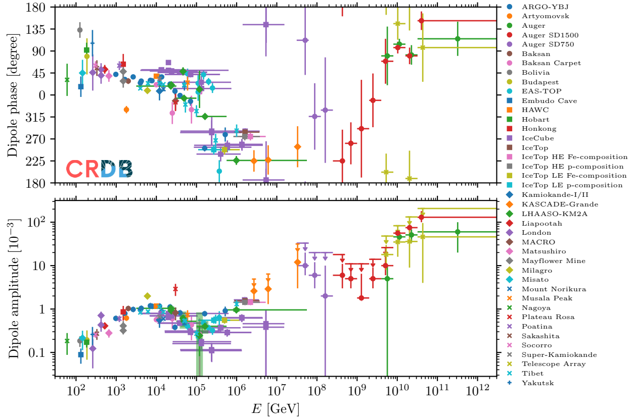
Figure 30.5: Phase and amplitude of the dipole anisotropy in CRs. Modified from Ref. [38].
