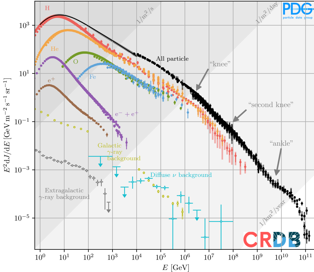
Figure 30.1: The spectrum of cosmic rays (CRs). Shown are measurements of the intensity of charged and neutral CRs, multiplied by kinetic energy squared. The data for the charged CRs [5–37] have been extracted from the Cosmic Ray Database (CRDB) [38] and we also include LHAASO data [39,40]. Below 10^4 GeV, the all-particle spectrum is the sum of spline fits of the most important nuclear species. The diffuse \gamma -ray fluxes have been extracted from Refs. [41–44], measurements of the diffuse neutrino background from Ref. [45]. Energy-integrated intensities are indicated by the various diagonal lines.
