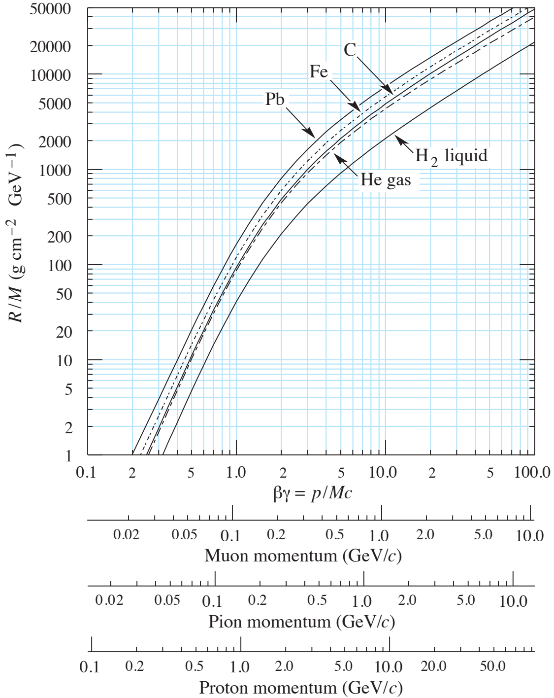
Figure 34.4: Range of heavy charged particles in liquid (bubble chamber) hydrogen, helium gas, carbon, iron, and lead. For example: For a K^+ whose momentum is 700 \text{ MeV}/c , \beta\gamma = 1.42 . For lead we read R/M \approx 396 , and so the range is 195 \text{ g cm}^{-2} (17 cm).
