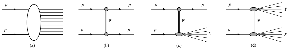
Figure 20.1: Schematic diagrams of soft pp processes. (a) non-diffractive processes, (b) elastic scattering, (c) single dissociation and (d) double dissociation. The double line corresponds to the Pomeron exchange.
